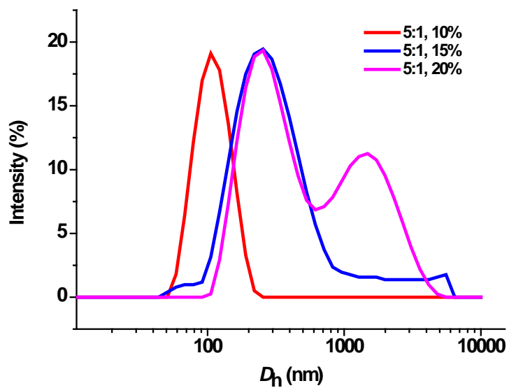
Fig. S1 DLS results of colloids synthesized at different solid contents while maintaining the mass ratio of styrene/CCS at 5:1.
