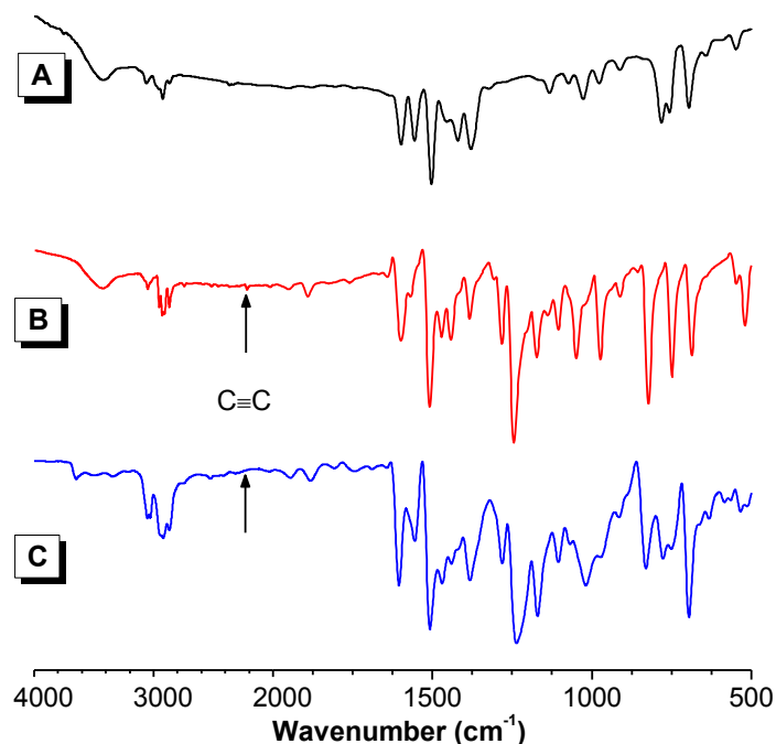
Fig. S1 IR spectra of (A) 1 , (B) 2(4) and (C) their polymer P1/2(4).
