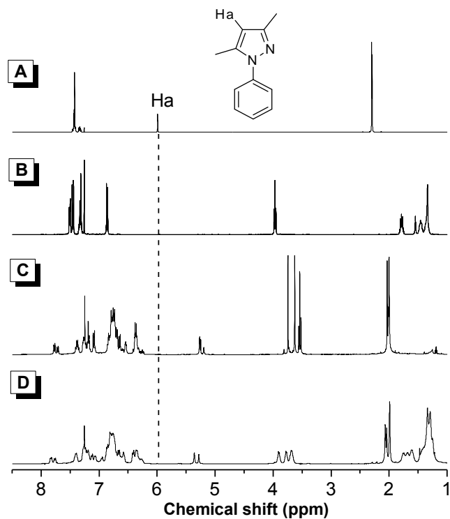
Fig. S6 ^1\text{H} NMR spectra of \text{CDCl}_3 solutions of (A) 1 , (B) 2(10) , (C) a mixture of 5–8 and (D) P1/2(10) (sample taken from Table 3, no. 4).
