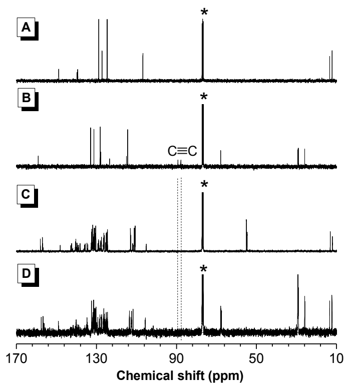
Fig. S7 ^{13}\text{C} NMR spectra of \text{CDCl}_3 solutions of (A) 1 , (B) 2(10) , (C) a mixture of 5–8 and (D) P1/2(10) (sample taken from Table 3, no. 4). The solvent peaks were marked with asterisks.
