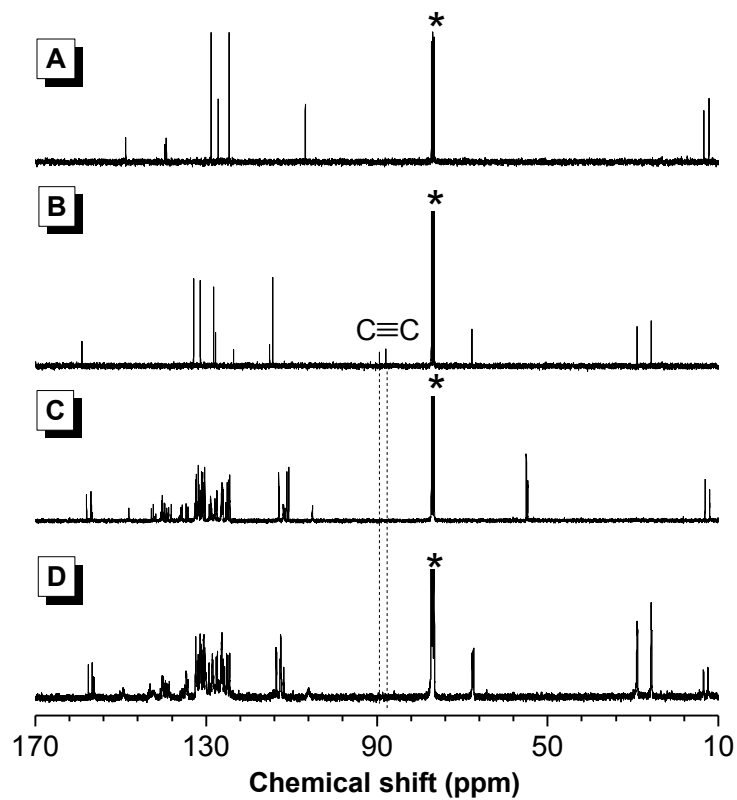
Fig. S3 13 C NMR spectra of CDCl 3 solutions of (A) 1 , (B) 2(6) , (C) a mixture of 5–8 and (D) P1/2(6) (sample taken from Table 3, no. 2). The solvent peaks were marked with asterisks.
