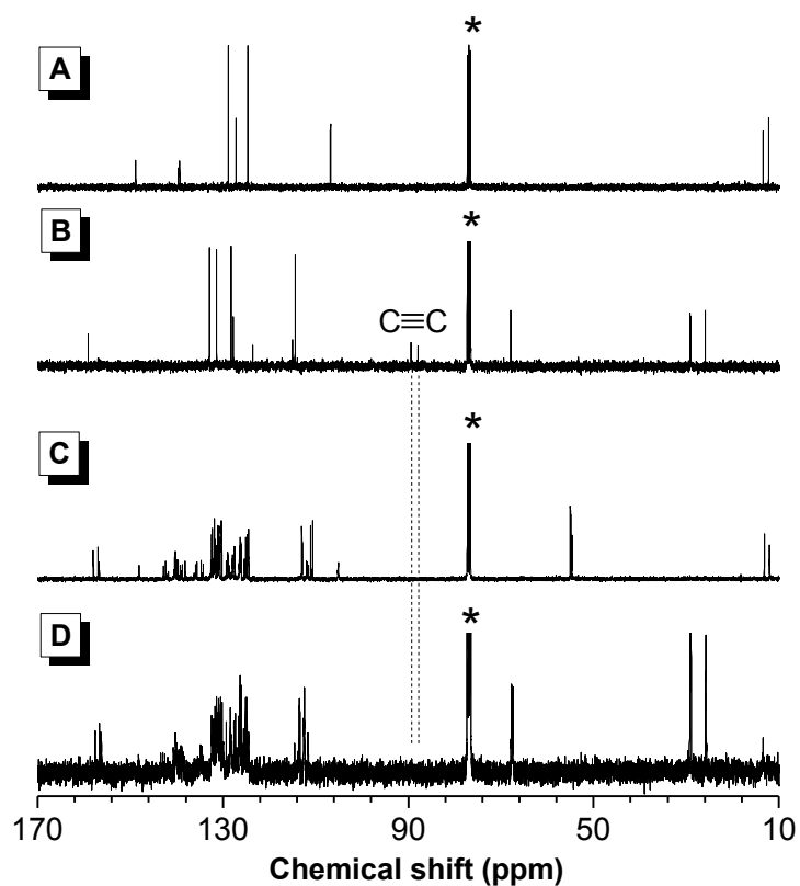
Fig. S5 13 C NMR spectra of CDCl 3 solutions of (A) 1 , (B) 2(8) , (C) a mixture of 5–8 and (D) P1/2(8) (sample taken from Table 3, no. 3). The solvent peaks were marked with asterisks.
