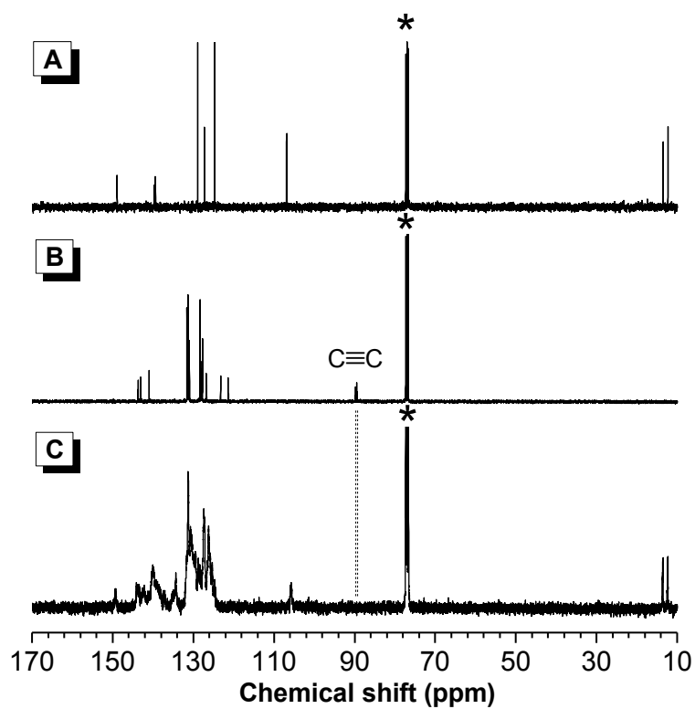
Fig. S9 ^{13}\text{C} NMR spectra of \text{CDCl}_3 solutions of (A) 1, (B) 3 and (C) P1/3 (sample taken from Table 3, no. 5). The solvent peaks were marked with asterisks.
