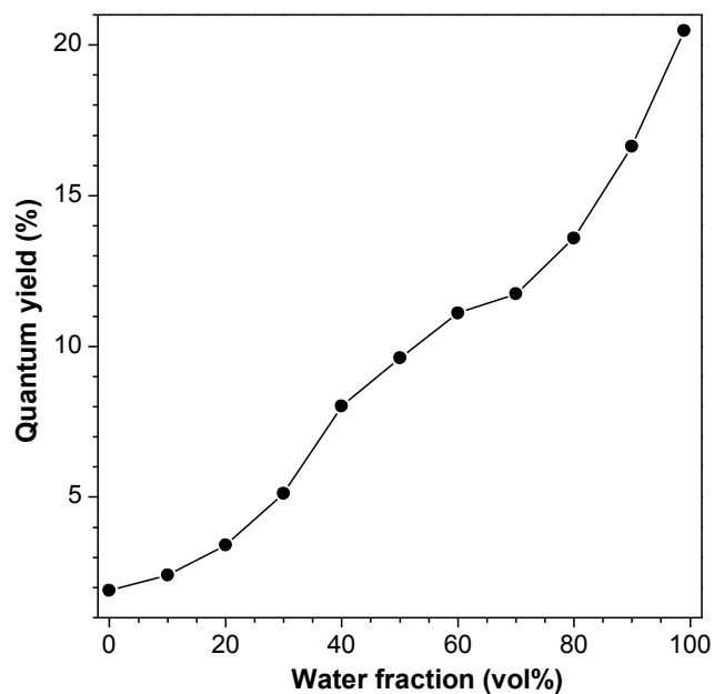
Fig. S11 Plot of quantum yield versus the solvent composition of THF/water mixture of P1/3.
