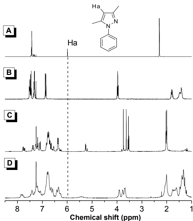
Fig. S4 1 H NMR spectra of CDCl 3 solutions of (A) 1 , (B) 2(8) , (C) a mixture of 5–8 and (D) P1/2(8) (sample taken from Table 3, no. 4).
