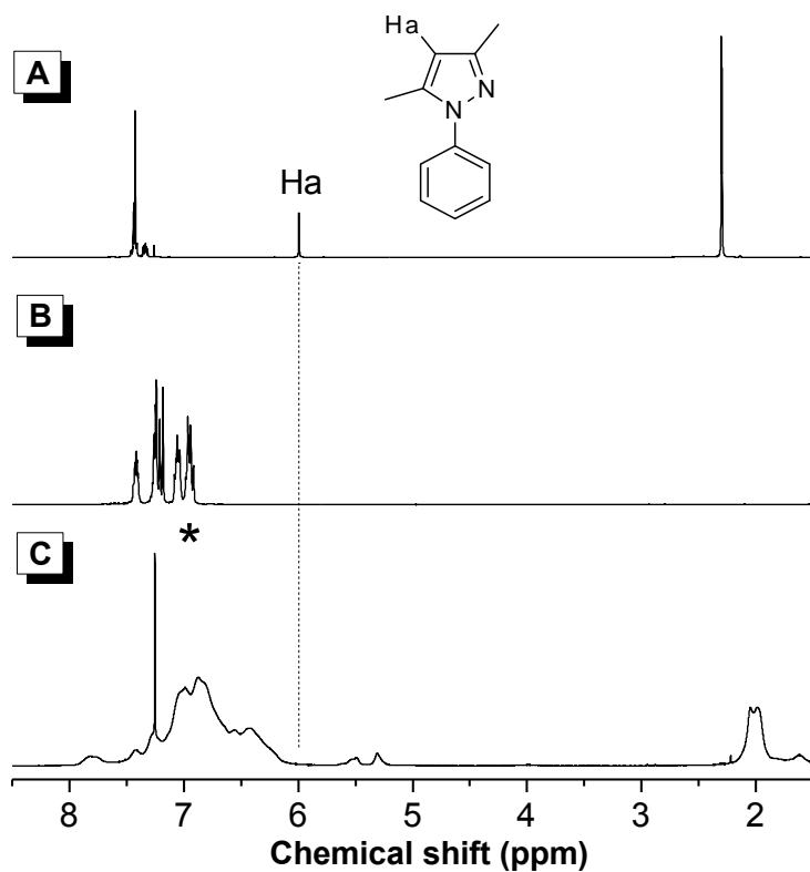
Fig. S8 ^1\text{H} NMR spectra of \text{CDCl}_3 solutions of (A) 1, (B) 3 and (C) P1/3 (sample taken from Table 3, no. 5).
