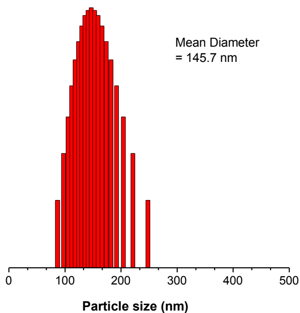
Fig. S10 Size distribution of nanoparticles of P1/3 suspended in 99% aqueous mixture. Concentration: 10 \mu M.
