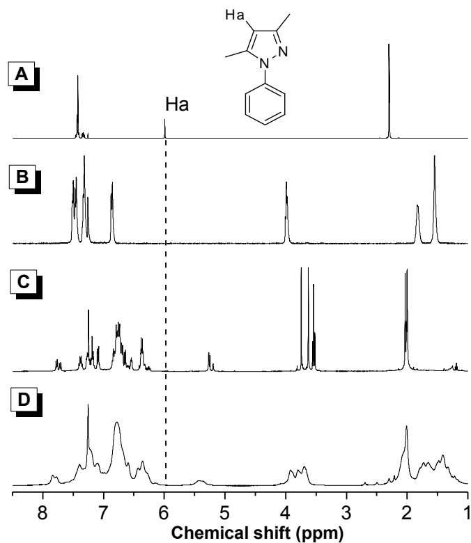
Fig. S2 1 H NMR spectra of CDCl 3 solutions of (A) 1 , (B) 2(6) , (C) a mixture of 5–8 and (D) P1/2(6) (sample taken from Table 3, no. 2).
