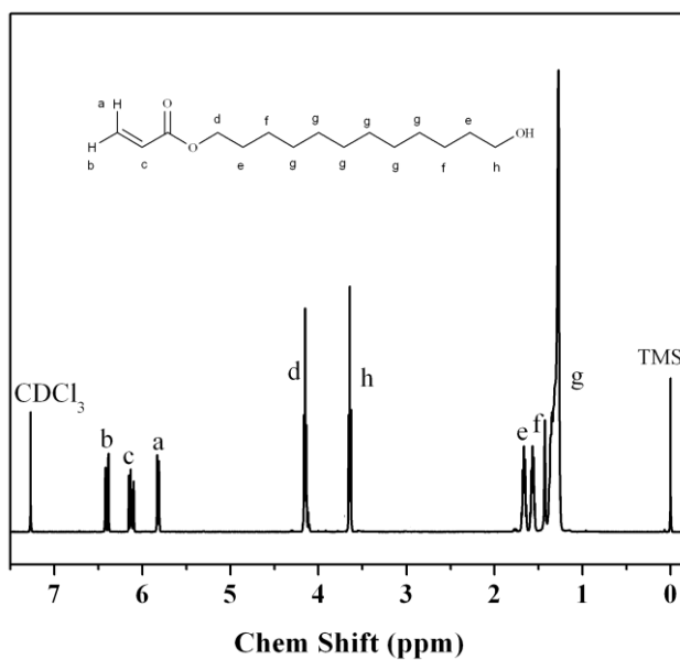
Figure S1. 1 H NMR spectrum of 12-hydroxydodecyl acrylate (CDCl 3 ).
