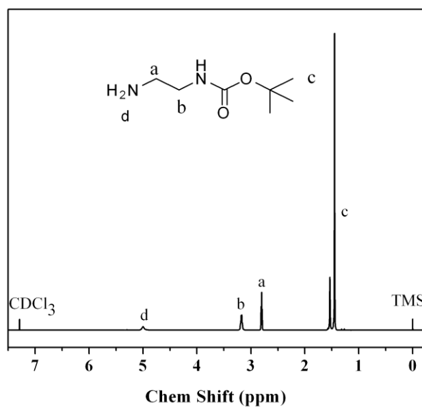
Figure S2. 1 H NMR spectrum of N -Boc-ethylenediamine (CDCl 3 ).
