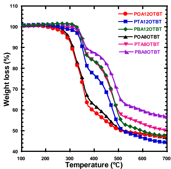
Figure S1. TG plots of POA12OTBT, PTA12OTBT, PBA12OTBT, POA8OTBT, PTA8OTBT, and PBA8OTBT
