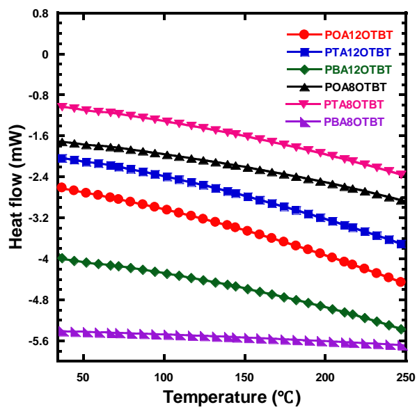
Figure S2. DSC plots of POA12OTBT, PTA12OTBT, PBA12OTBT, POA8OTBT, PTA8OTBT, and PBA8OTBT
