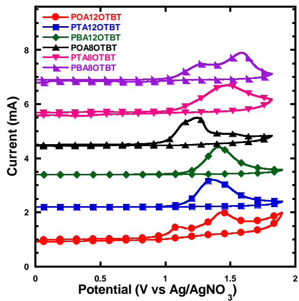
Figure S3. Cyclic voltammograms of the copolymers films measured in 0.1 M Bu 4 NPF 6 in acetonitrile at a scan rate of 50 mVs -1 .
