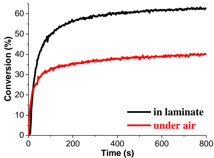
Figure S1. Photopolymerization profiles of Ebecryl 605 (from Cytec) in the presence of MANA_1/Iod/NVK (1%/2%/3%, w/w/w) in laminate and under air upon the laser diode at 457 nm exposure.
