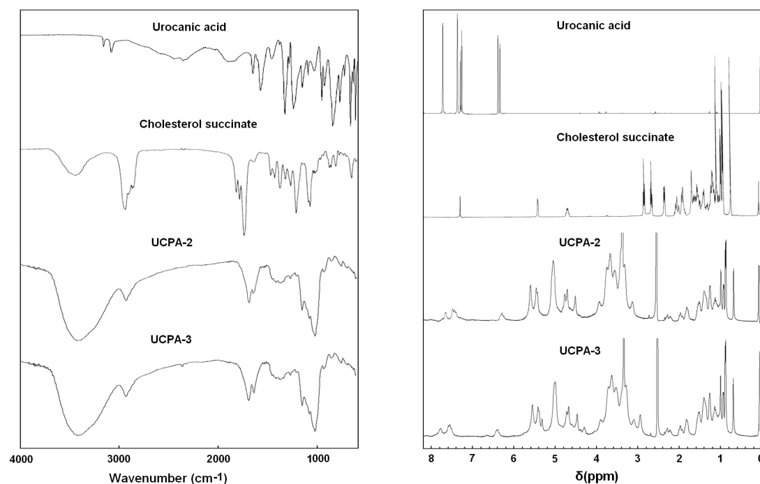
Fig. S1 IR (a) and 1 H NMR spectra (b) of urocanic acid, cholesterol succinate, UCPA-2, and UCPA-3.
