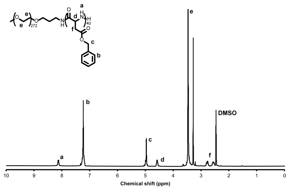
Fig. S1. ^1\text{H} NMR spectrum of PEG- b -PBLA in \text{DMSO-}d_6 at 25 °C.
