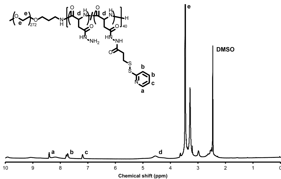
Fig. S2. ^1\text{H} NMR spectrum of PEG- b -P[Asp(PDP x )] in DMSO- d 6 at 25 °C.
