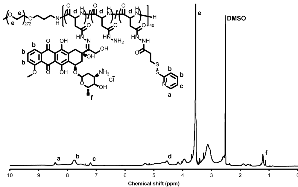
Fig. S3. ^1\text{H} NMR spectrum of PEG- b -P[Asp(PDP x /Hyd-DOX y )] in DMSO- d 6 at 70 °C.
