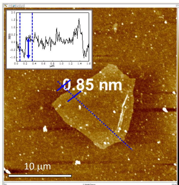
Fig. S1. AFM image of as-synthesized graphene nanosheets. The inset shows the depth profile of graphene nanosheets, which gave a thickness of 0.85nm. The size of graphene nanosheets is about 10 μm x 10 μm.
