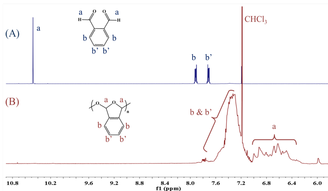
Figure SI 1, 1 H NMR spectra (CDCl 3 , 21°C, 400MHz) of both PA monomer (A) and corresponding crude PPA 5 sample (B).
