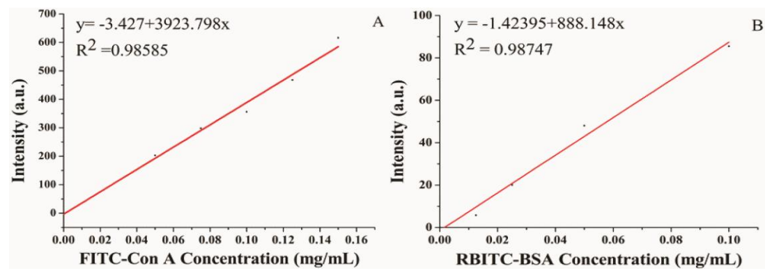
Figure S4. Calibration curve of (A): FITC-Con A; (B): RBITC-BSA
