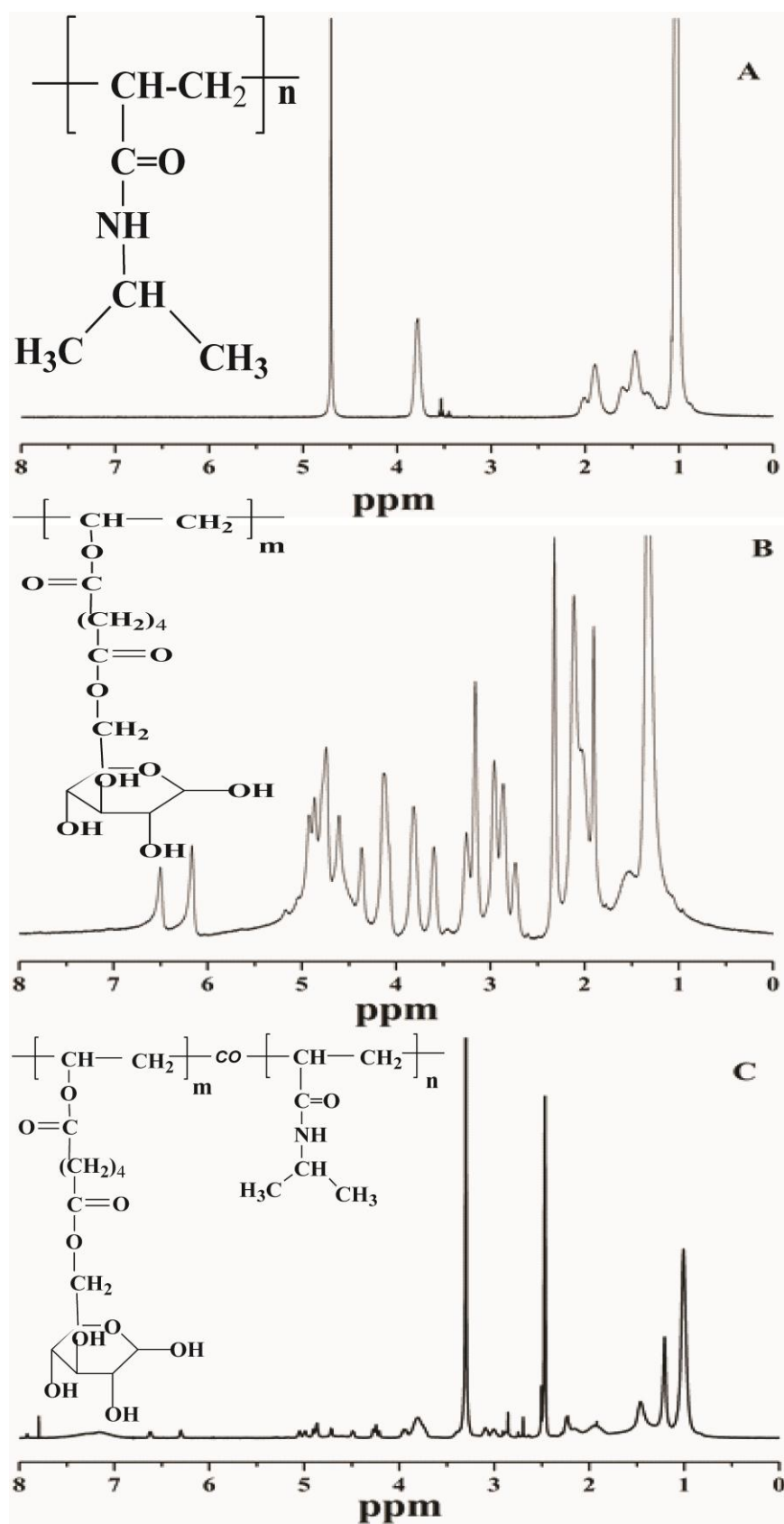
Figure S2. ^1\text{H} NMR spectra of (A) PNIPAM; (B) Poly-OVDG; (C) PND-3 (OVDG: NIPAM ratio 1:15).
