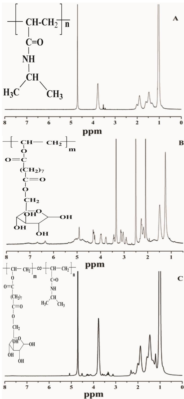
Figure S3. ^1\text{H} NMR spectra of (A) PNIPAM; (B) Poly-OVZG; (C) PNZ-1 (OVZG : NIPAM ratio 1:7).
