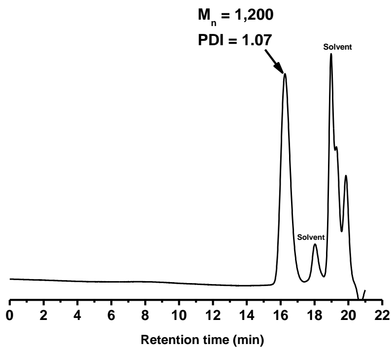
Figure S1. GPC curve of control experiment product only with DHPEG ( M_n = 1000 ) in the presence of \text{Sc}(\text{OTf})_3 under the same conditions (120 °C, 0.3-3 mmHg, 12 h).
