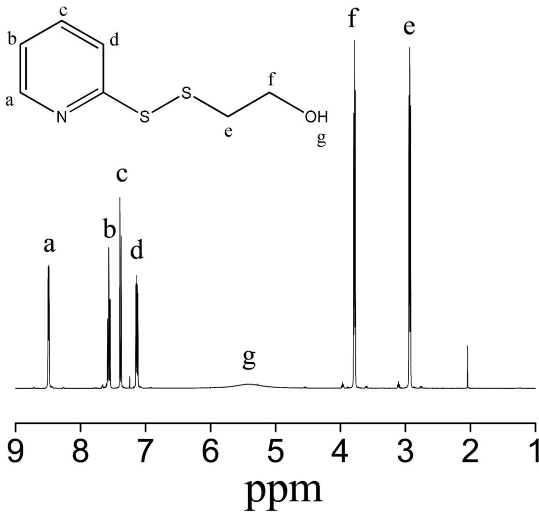
Fig. S1. ^1\text{H} NMR spectrum of hydroxyethyl pyridyldisulfide (Compound 1) in \text{CDCl}_3 solvent (400 MHz).
