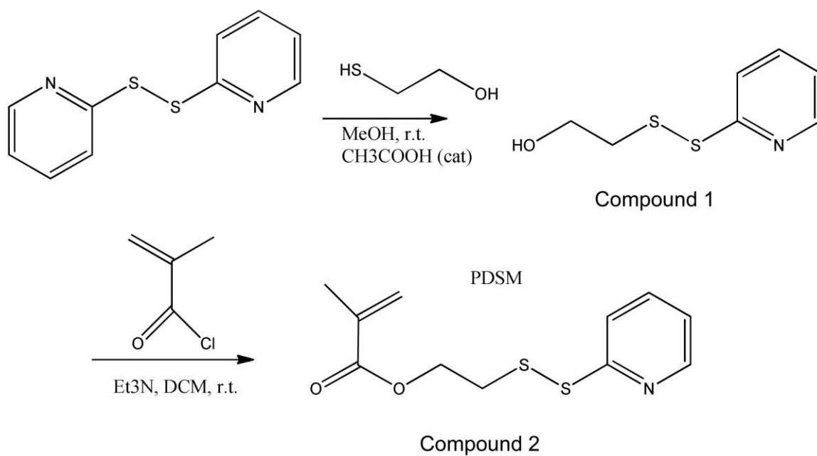
Scheme S1. Synthesis of pyridyldisulfide ethymethacrylate (PDSM).
