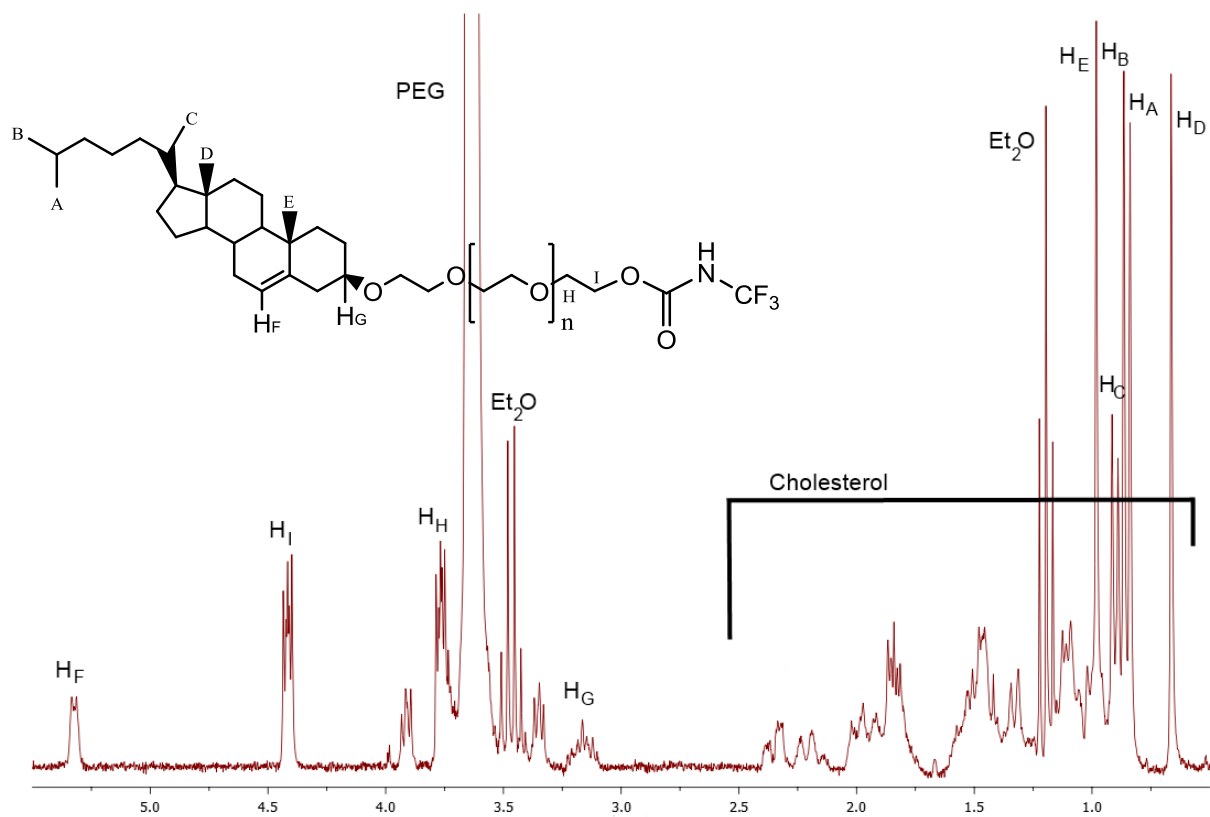
Figure S2. FT-IR spectrum of N -( tert -butoxycarbonyl)-6- O -(3-mercaptopropanoyl)-D-glucosamine
