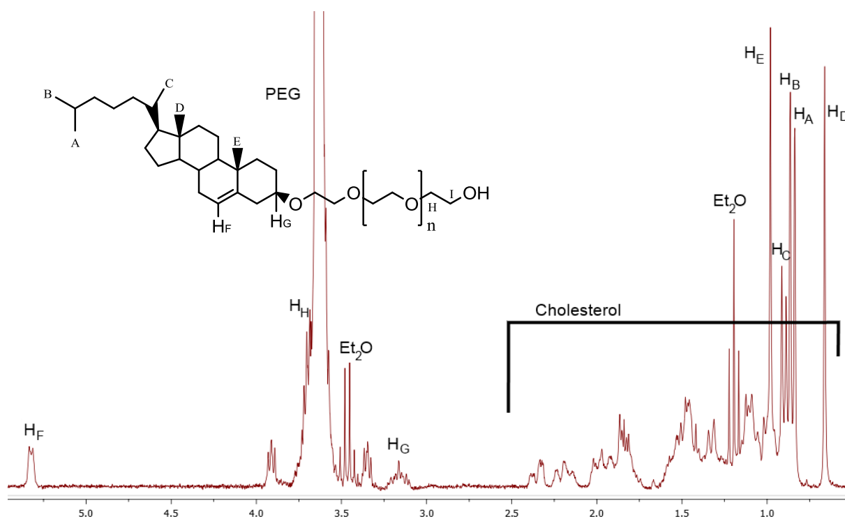
Figure S1. 1 H NMR spectra of cholesterol-PEG-OH, and after reaction with trifluoromethyl isocyanate
