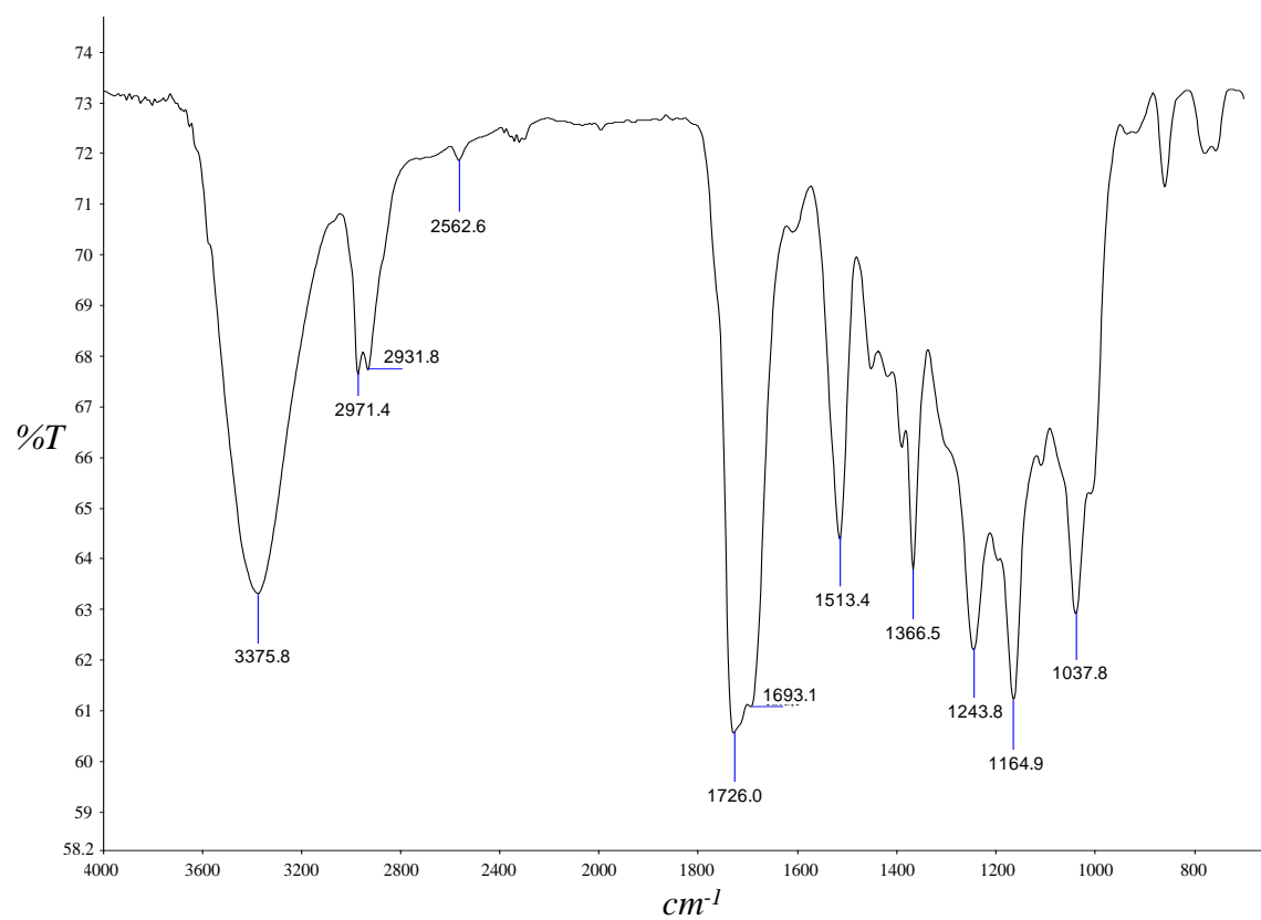
Figure S2. FT-IR spectrum of N -( tert -butoxycarbonyl)-6- O -(3-mercaptopropanoyl)-D-glucosamine
