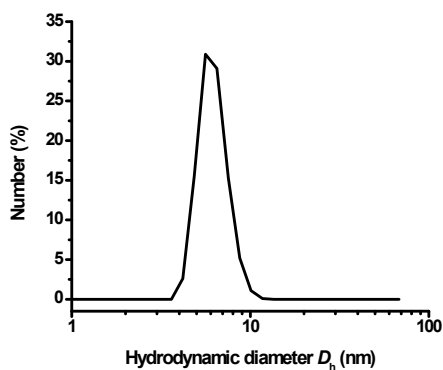
Fig. S1 DLS of the polymer synthesized under conditions: solid content 10% w/v, 70 °C, 4 h, molar ratio of CTA:PEGMA2K:V-50 = 1:5:0.2, [PBS] = 0.15 M.
