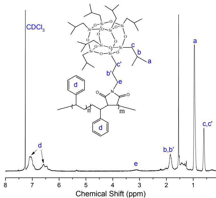
Figure S2. The ^1\text{H} NMR spectrum of PSMIPOSS 18 - b -PS 109 block copolymer.
