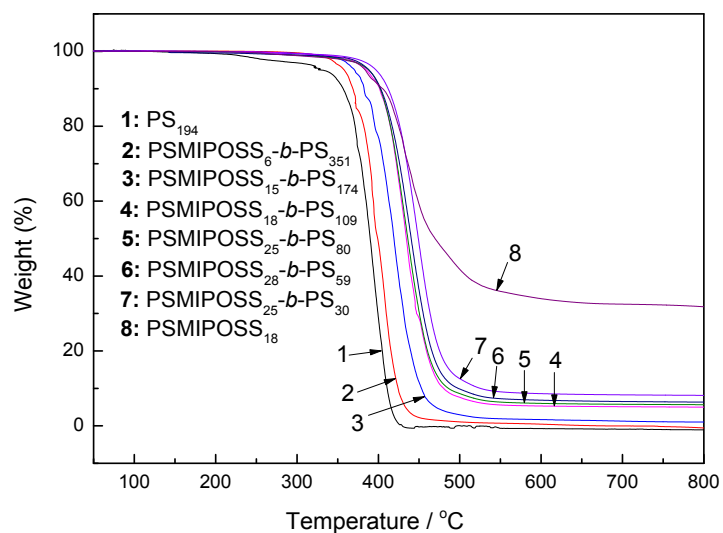
Figure S4. TGA curves of PS, PSMIPOSS and PSMIPOSS- b -PS copolymers.
