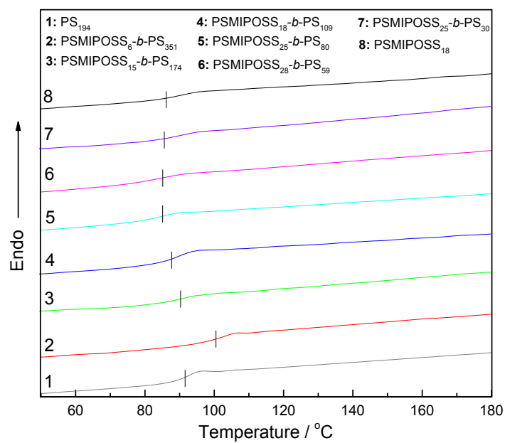
Figure S5. DSC thermograms of PS, PSMIPOSS and PSMIPOSS- b -PS copolymers.
