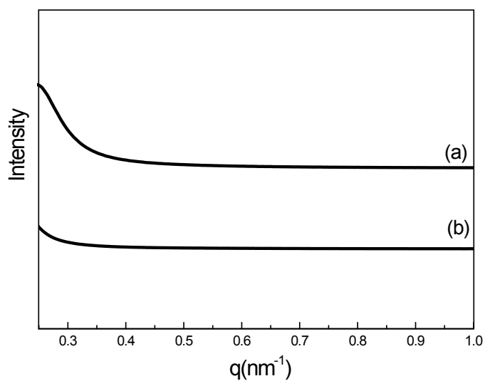
Figure S3. Small-angle X-ray scattering (SAXS) curves of (a) PSMIPOSS 28 - b -PS 59 and (b) PSMIPOSS 25 - b -PS 30 .
