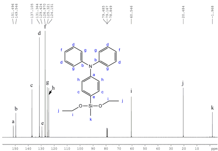
Figure S2. 13 C NMR spectrum of 4-(diethoxy(methyl)silyl)-N,N-diphenylaniline
