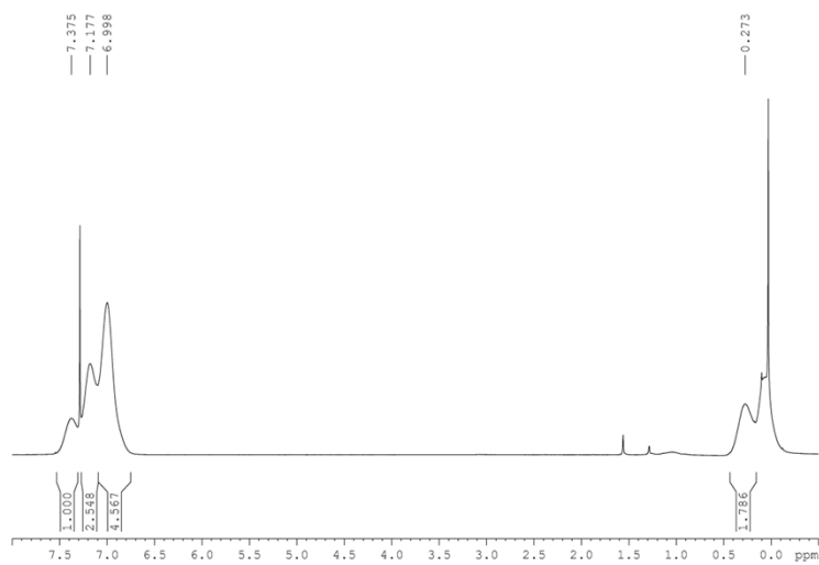
Figure S4. ^1\text{H} NMR spectrum of PTPAMSi
