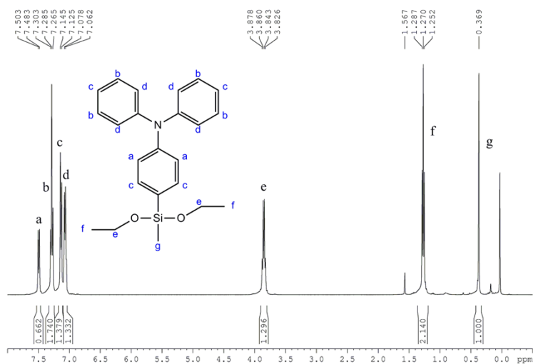
Figure S1. 1 H NMR spectrum of 4-(diethoxy(methyl)silyl)-N,N-diphenylaniline
