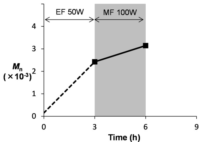
Figure S2. Solution polycondensation of L-LA catalyzed by \text{Sc}(\text{OTf})_3 under alternating irradiation of EF (50 W) and MF (100 W).
