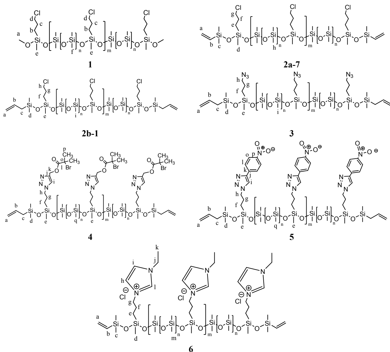
Figure S1: Structures for ^{13}\text{C} -NMR assignment.
