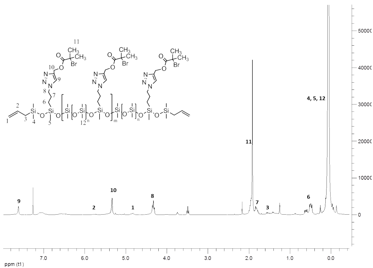
Figure S2: 1 H-NMR spectrum of 4.
