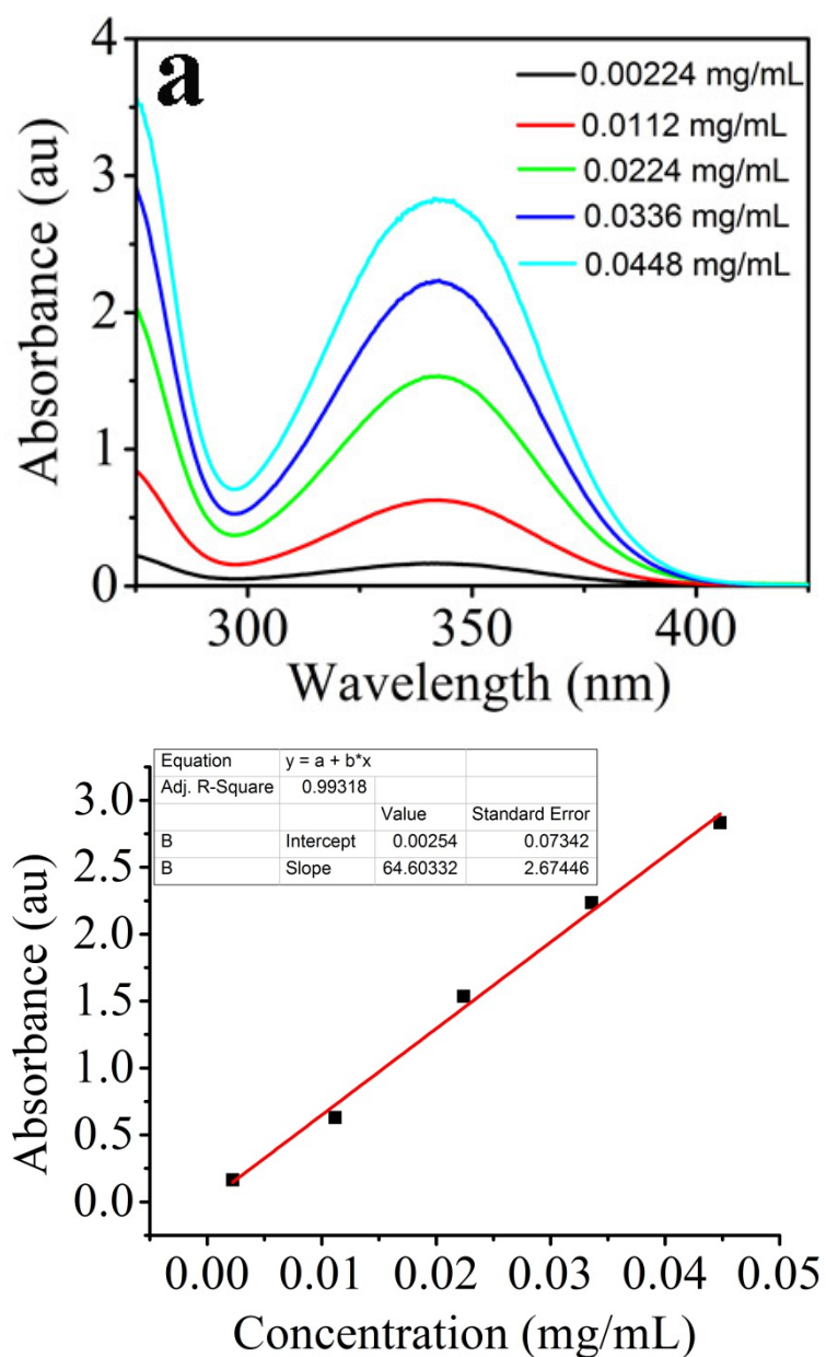
Figure S2. (a) Absorptions of pyridine-2-thione in PBS buffer solution at different concentrations, (b) a standard curve of absorbance of pyridine-2-thione vs. concentration.
