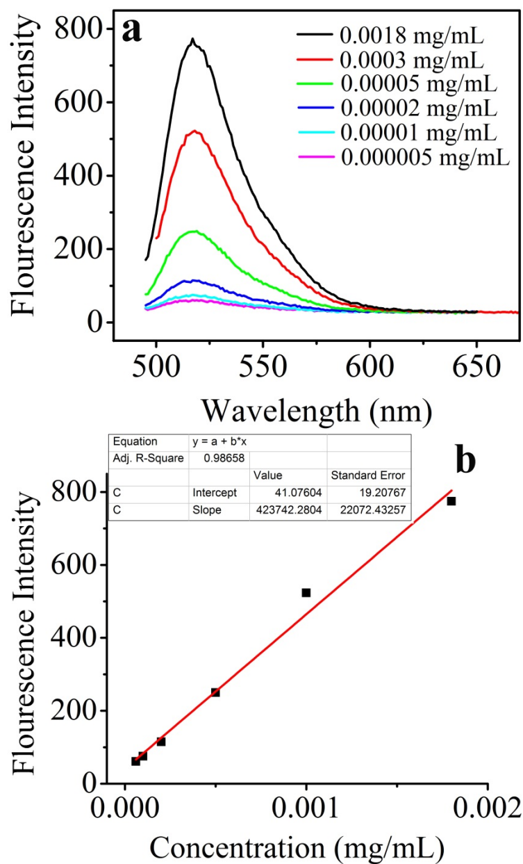
Figure S3. (a) Emission spectra of FITC recorded at different concentrations in buffer solution, (b) a plot of intensity of fluorescence emission of FITC vs. concentration.
