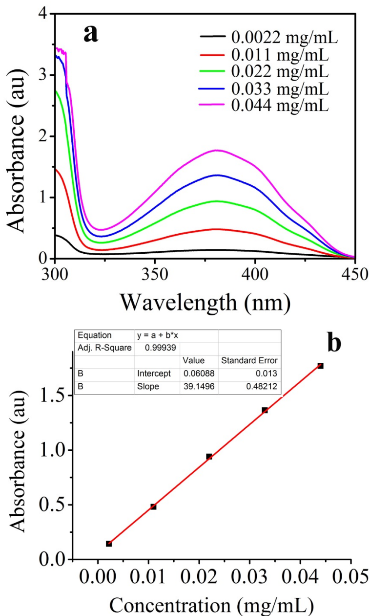
Figure S1. (a) Absorptions of pyridine-2-thione in THF at different concentrations, (b) a standard curve of absorbance of pyridine-2-thione vs. concentration in THF.
