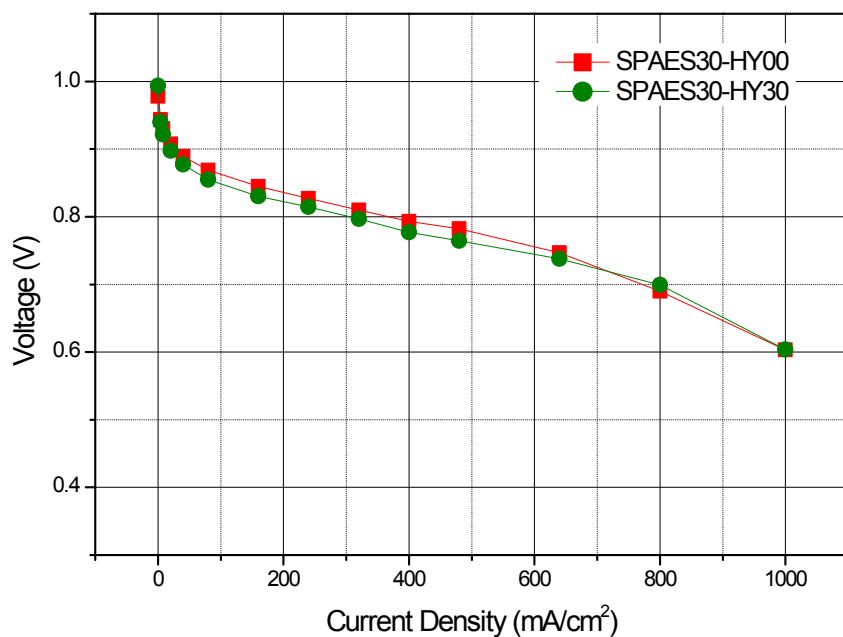
Figure S1. Polarization curves of SPAES30-HY00 and SPAES30-HY30, excluding the effect of ohmic resistance.
