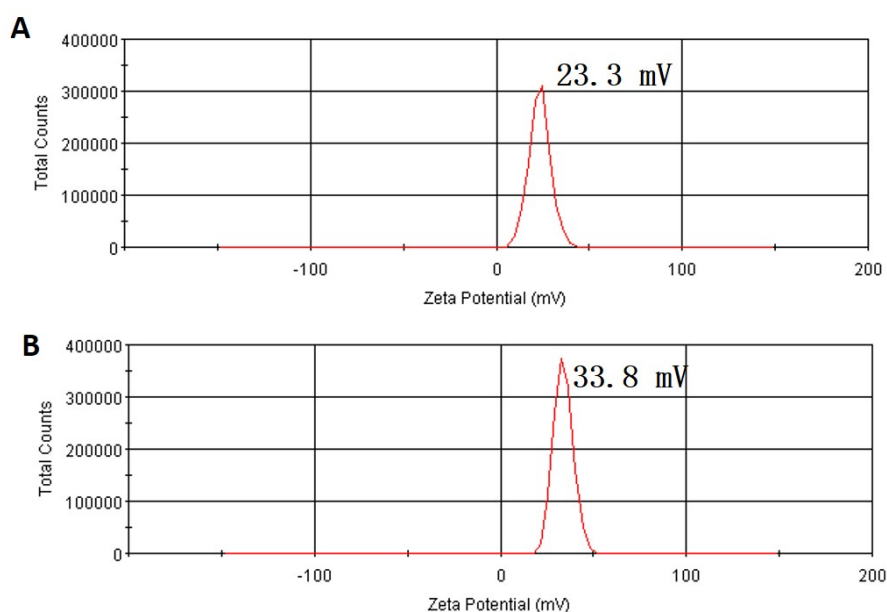
Fig. S1 Zeta potential ( \zeta ) of Fe 3 O 4 @SiO 2 -PDMAEMA aqueous solution before (A) and after (B) CO 2 treatment.
