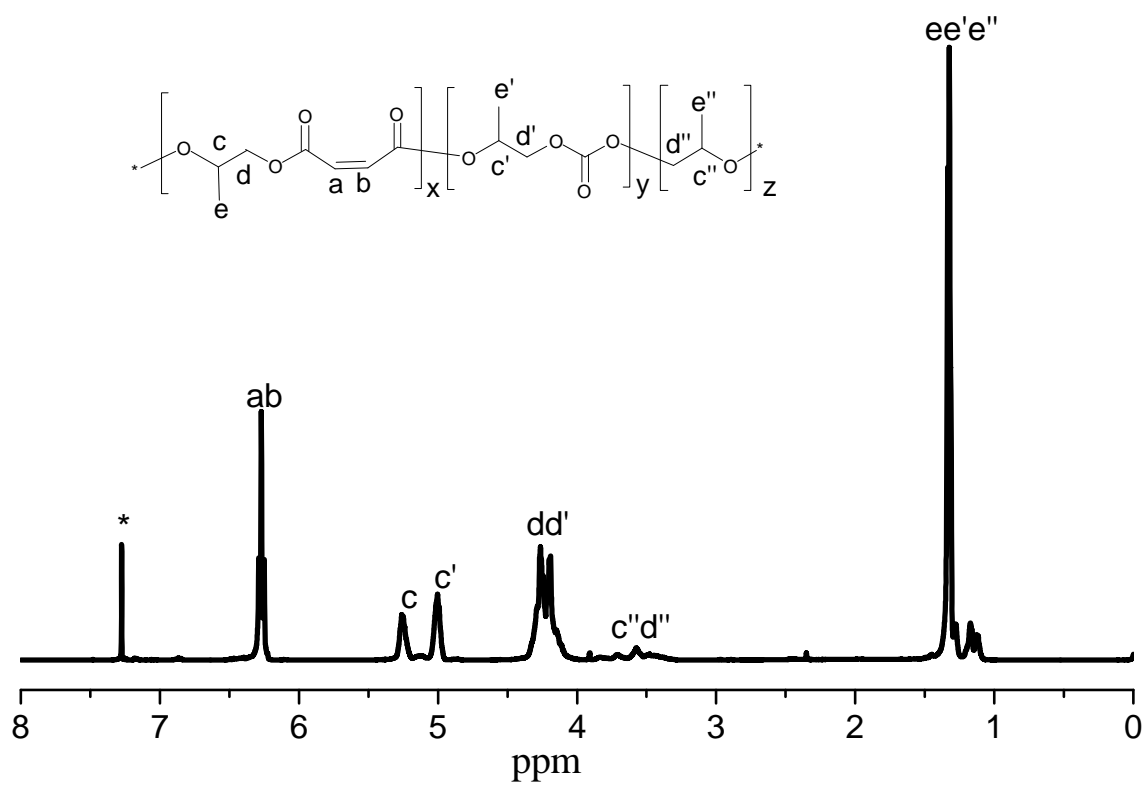
Fig.S2 1 H NMR spectrum of MA/PO/CO 2 terpolymer
