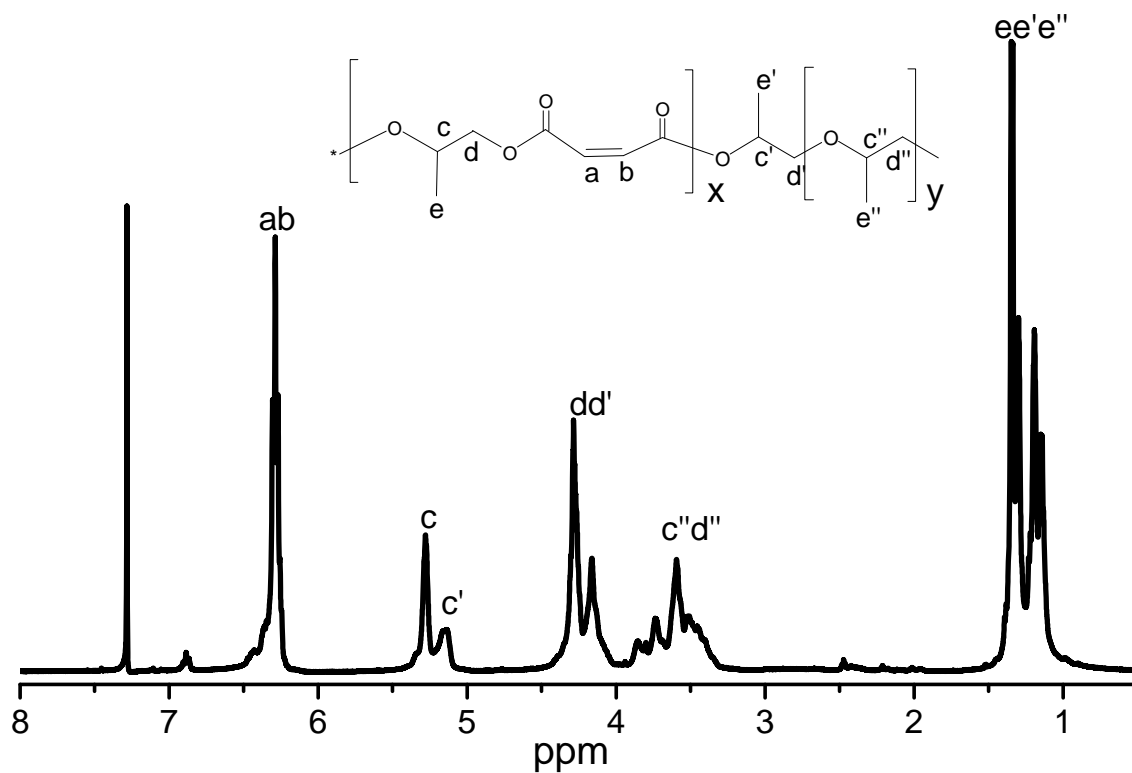
Fig.S1 1 H NMR spectrum of PO/MA copolymer
