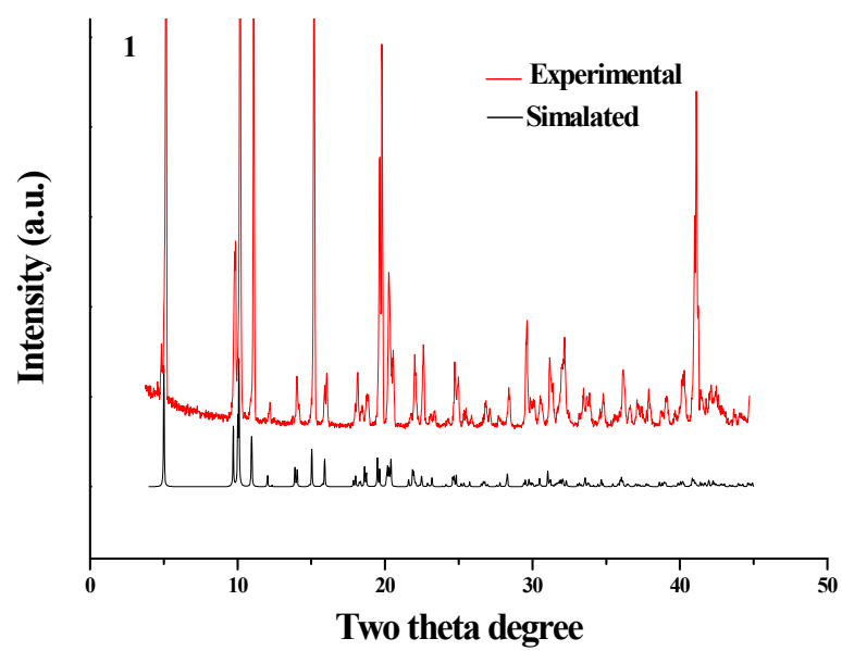
Fig. S3 Powder XRD pattern of 1.
