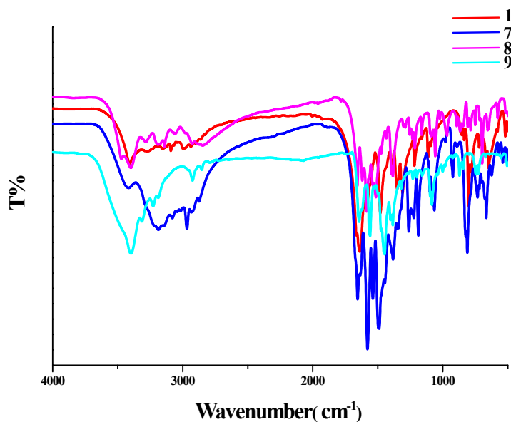
Fig. S1 IR spectra of title compounds.
