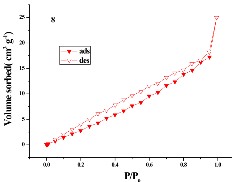
Fig. S2 \text{N}_2 adsorption-desorption isotherms of 8 at 77 K.
