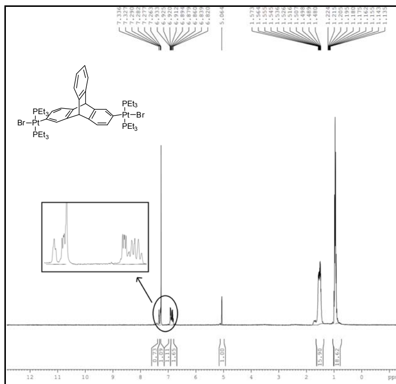
^1\text{H} NMR spectrum of 1 .
