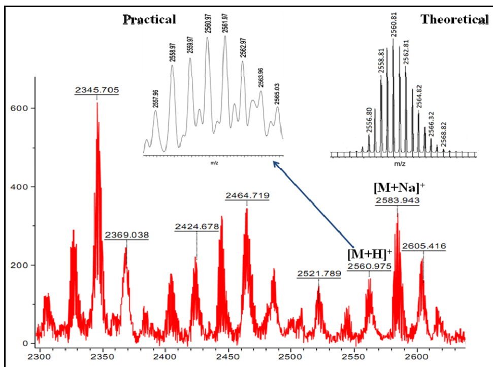
MALDI-TOF-MS data of 5 .
