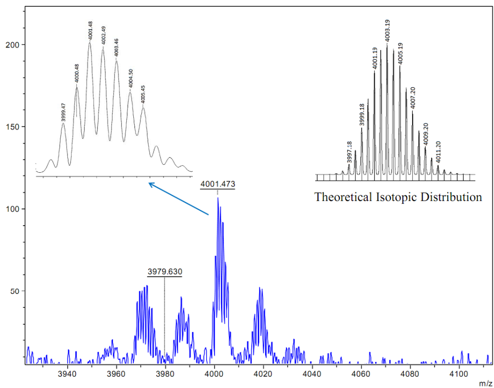
MALDI-TOF-MS data of 6 .
