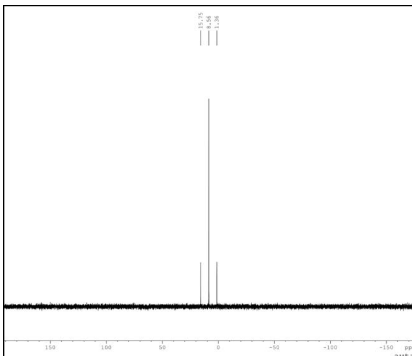
^{31}\text{P} NMR spectrum of 2 .
