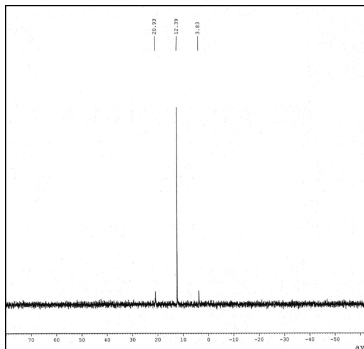
^{31}\text{P} NMR spectrum of 1 .
