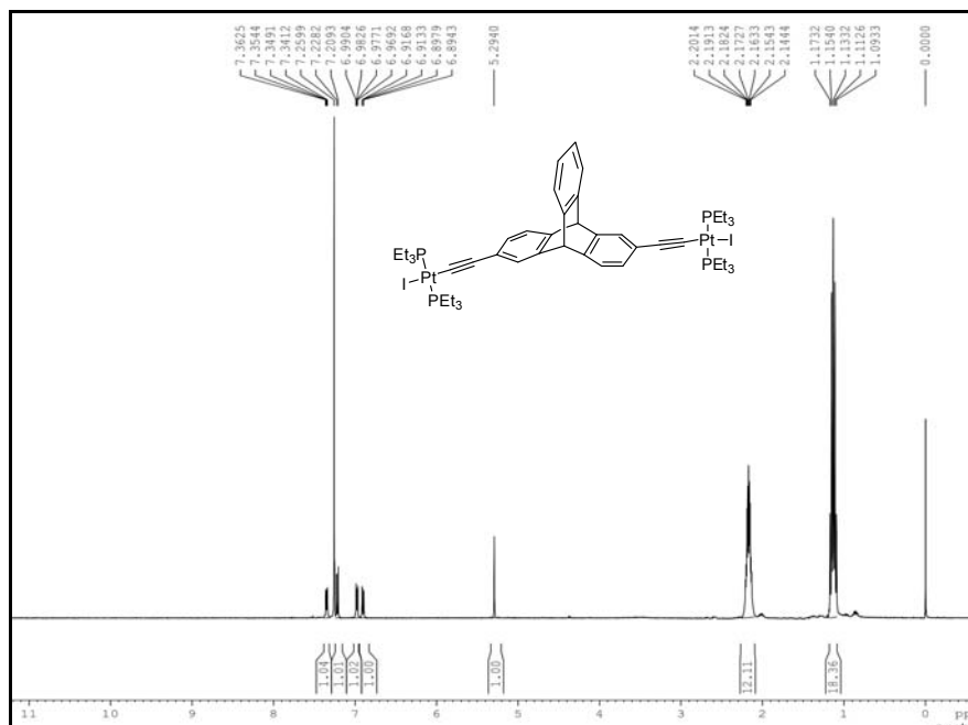
^1\text{H} NMR spectrum of 2 .
