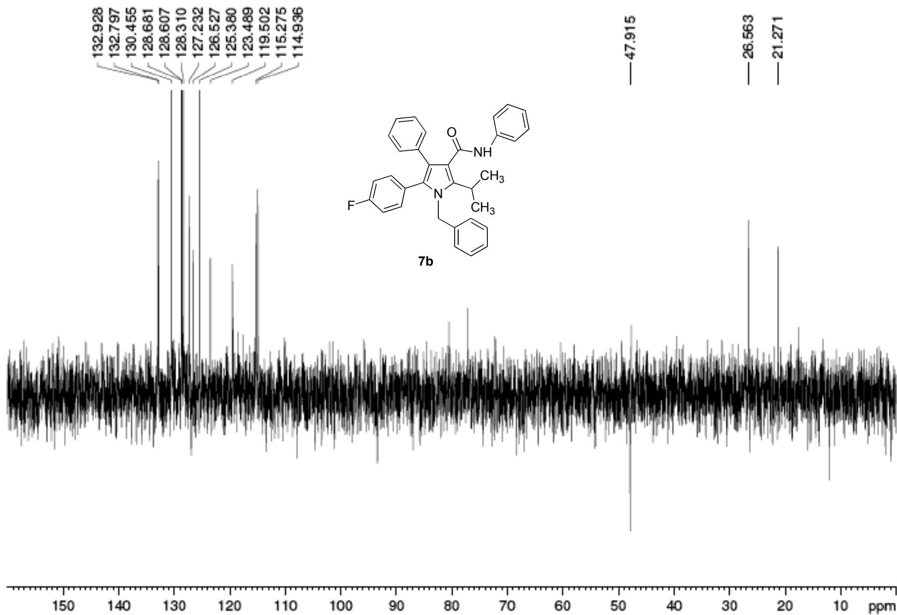
DEPT-135 spectrum of compound 7b
