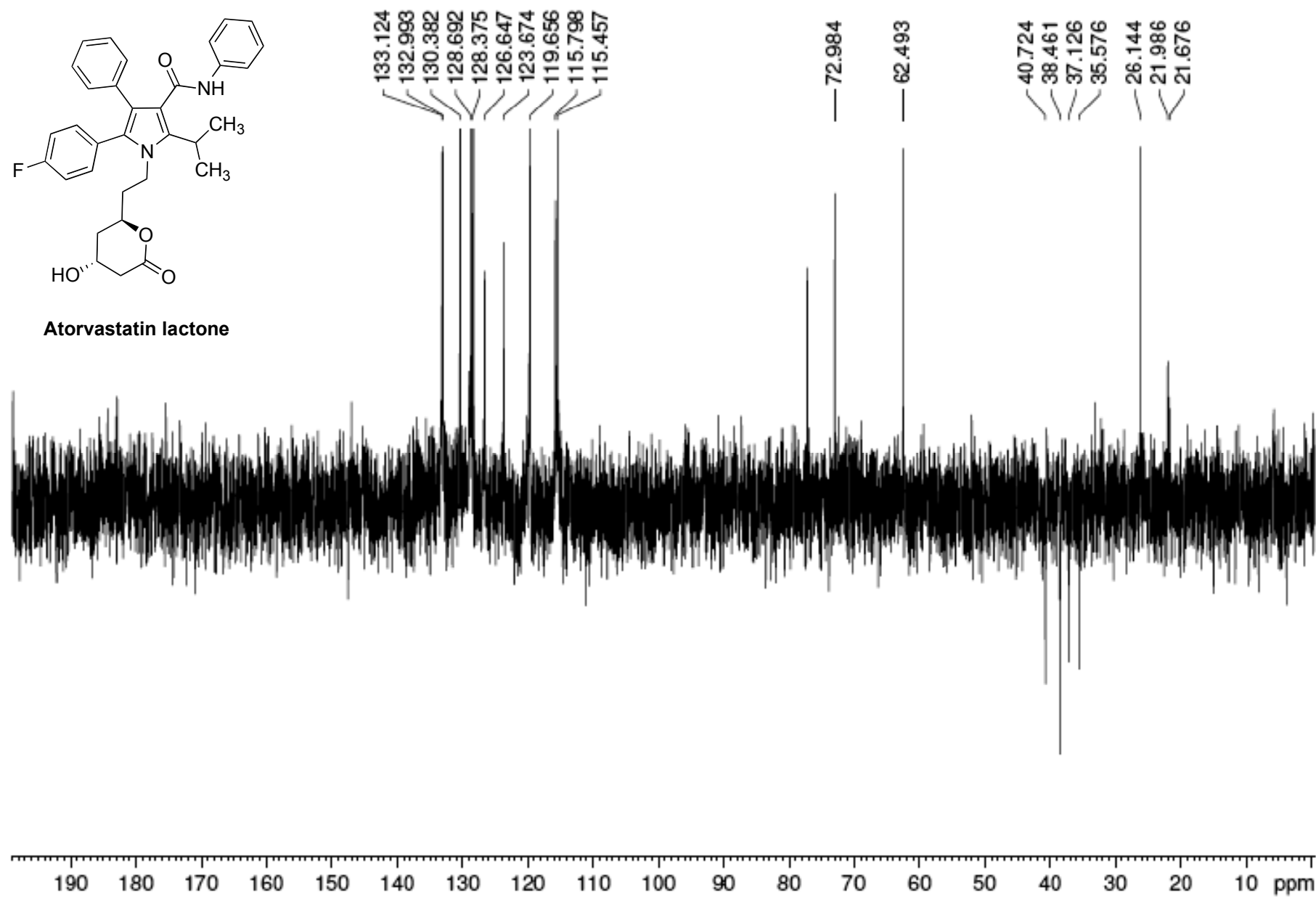
DEPT-135 spectrum of atorvastatin lactone (9)
