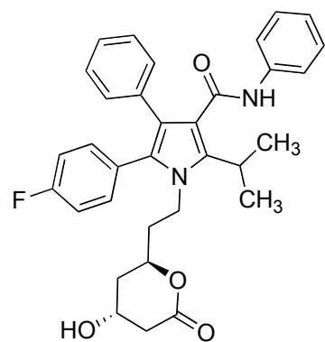
Atorvastatin lactone
