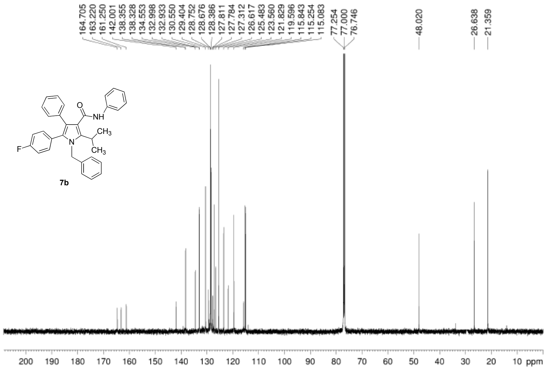
^{13}\text{C} NMR spectrum of compound 7b
