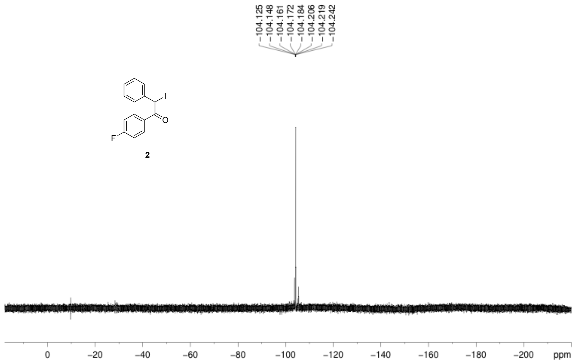
^{19}\text{F} NMR spectrum of compound 2
