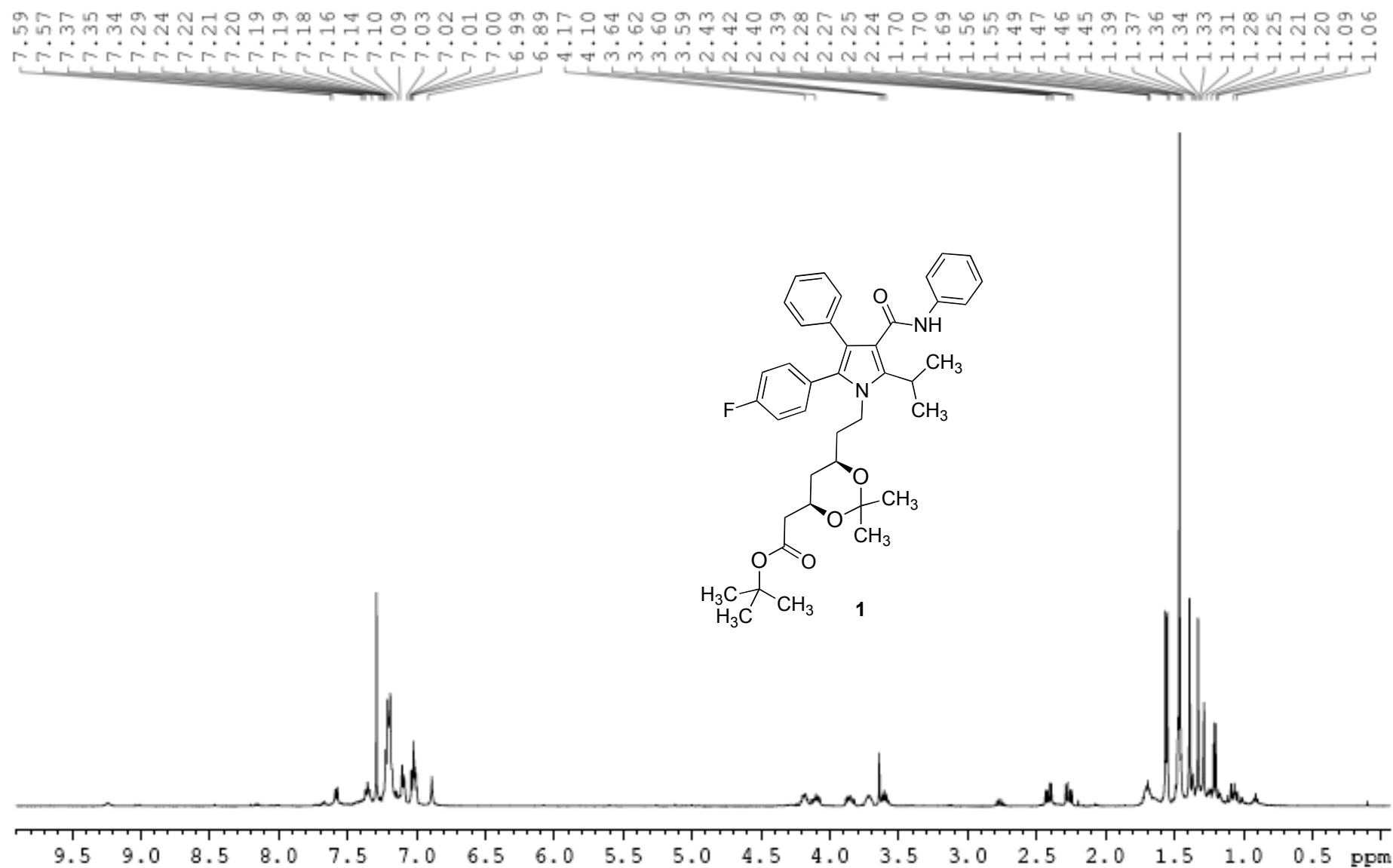
1 H NMR spectrum of compound 1
