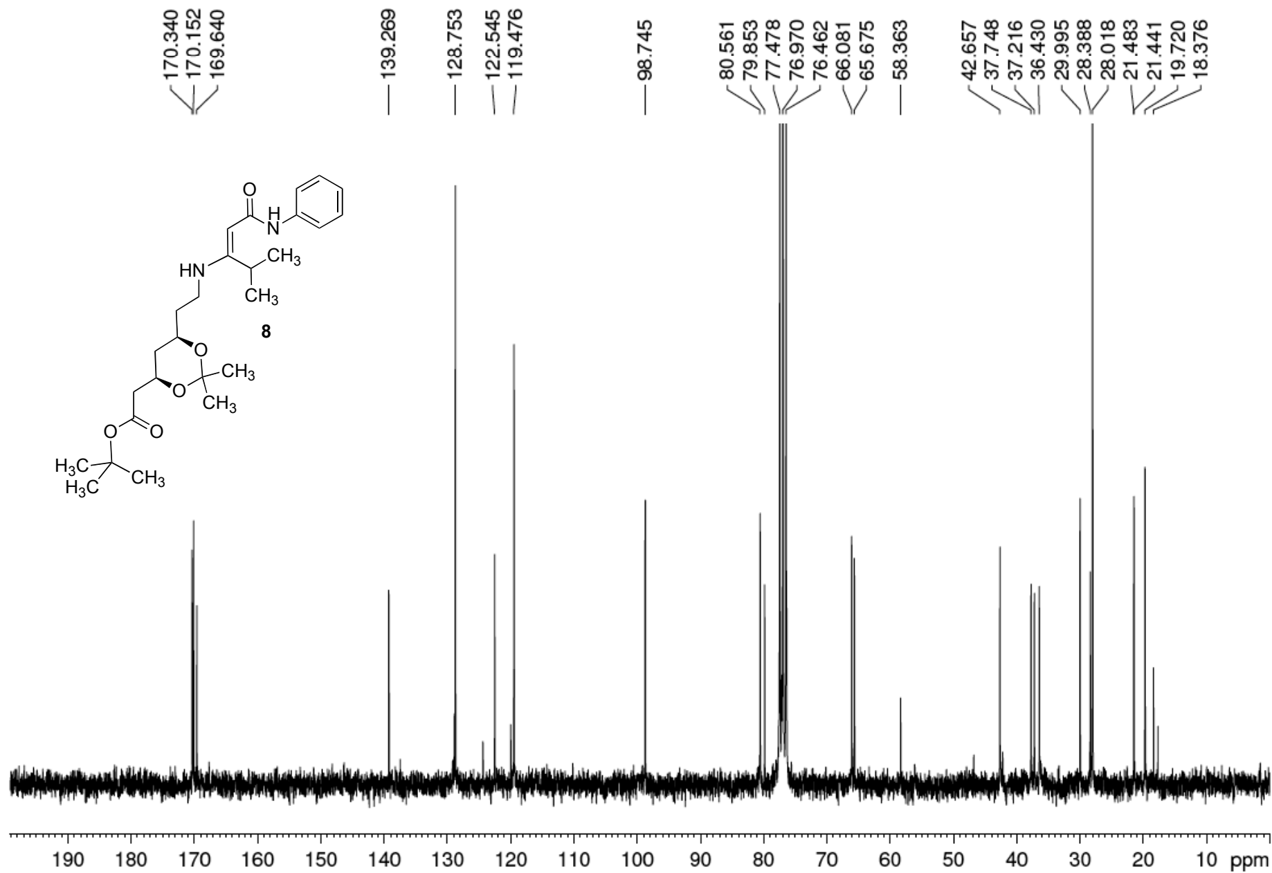
13 C NMR spectrum of compound 8
