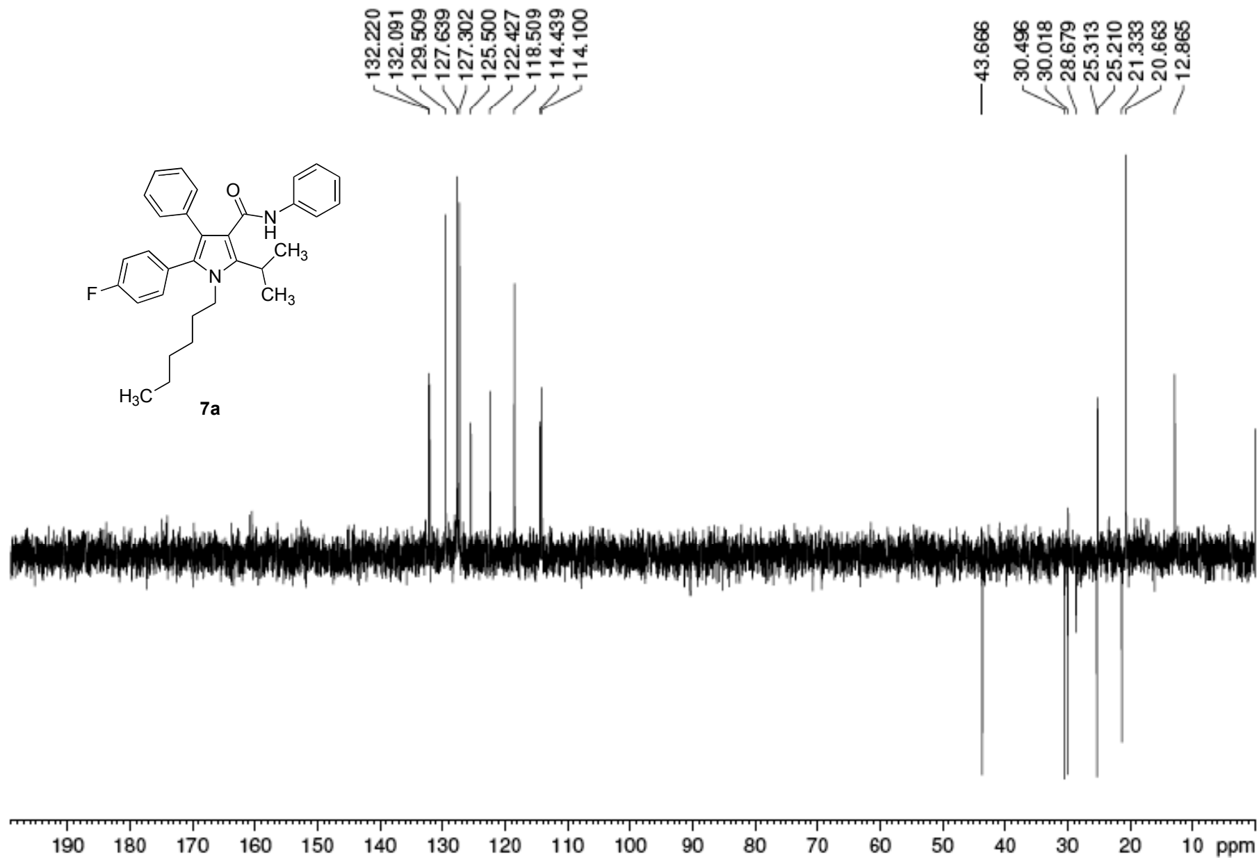
DEPT-135 spectrum of compound 7a
