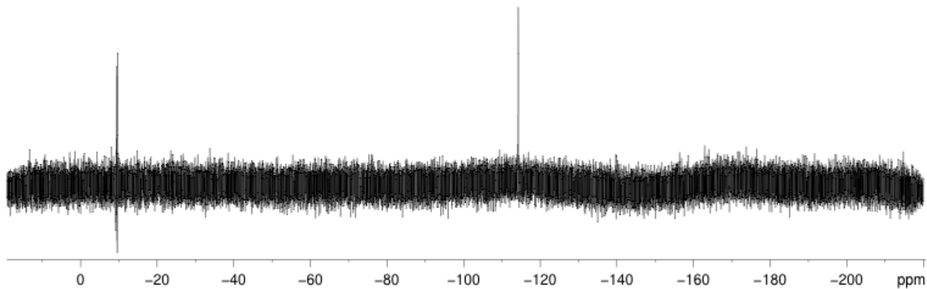
^{19}\text{F} NMR spectrum of compound 7a
