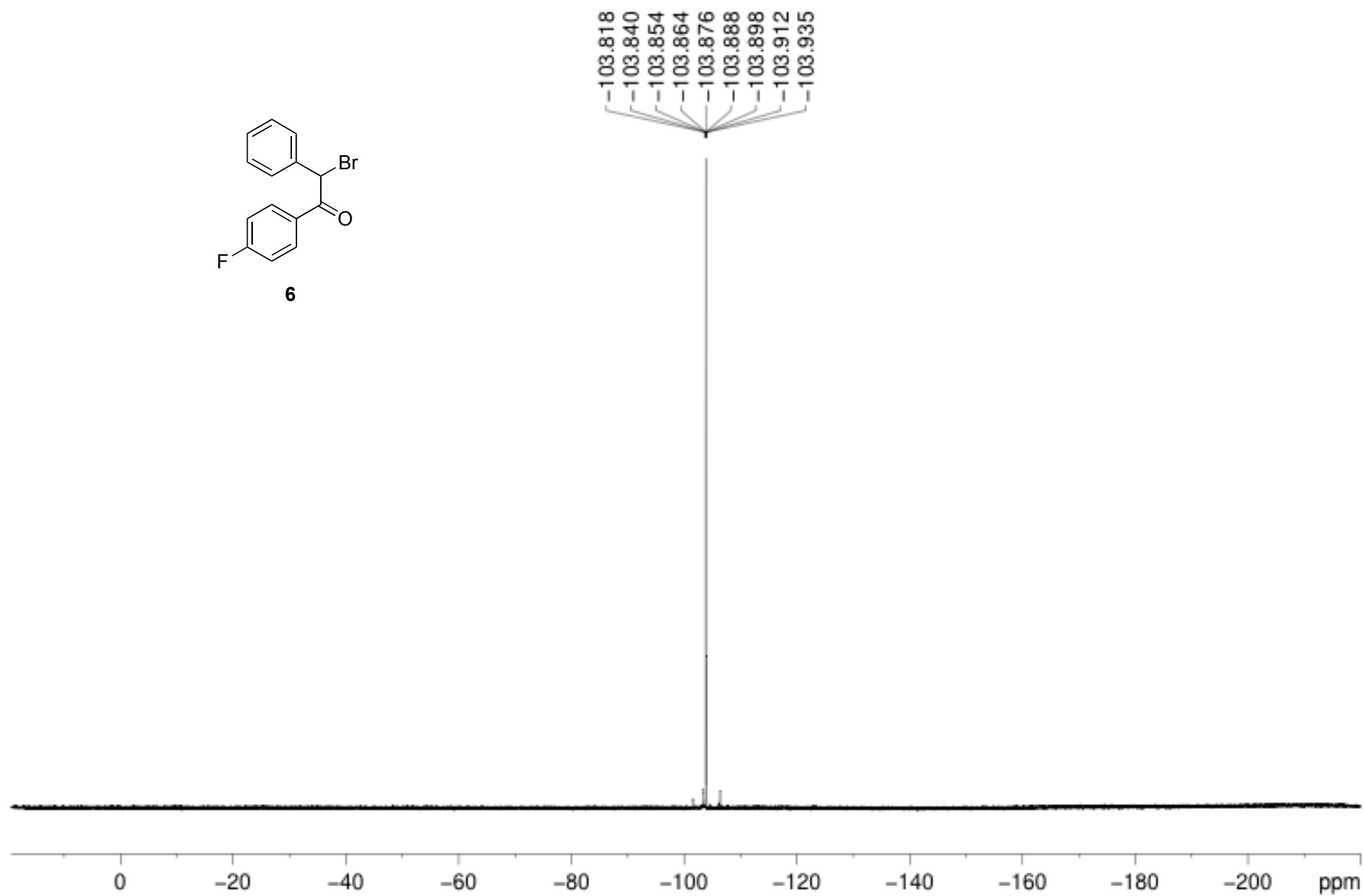
^{19}\text{F} NMR spectrum of compound 6
