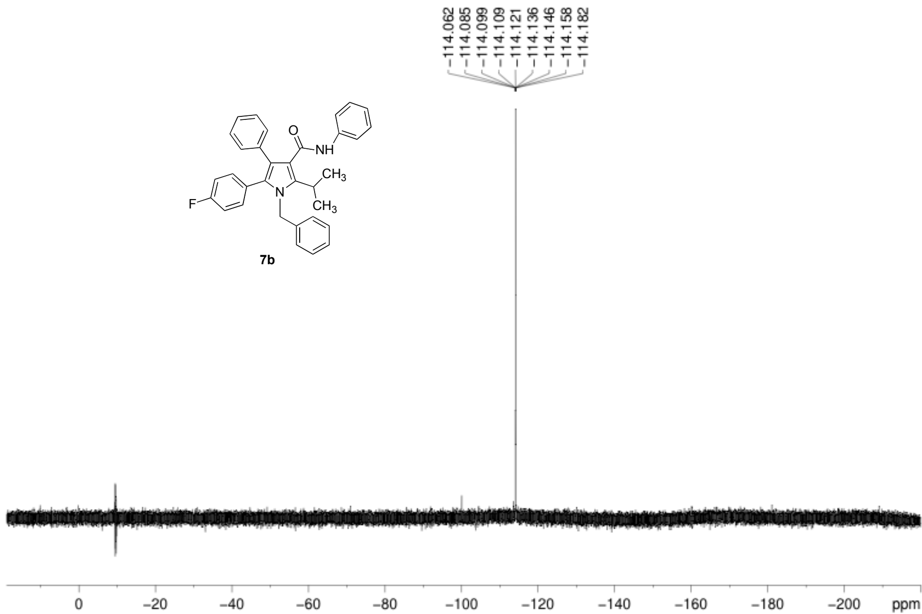
^{19}\text{F} NMR spectrum of compound 7b
