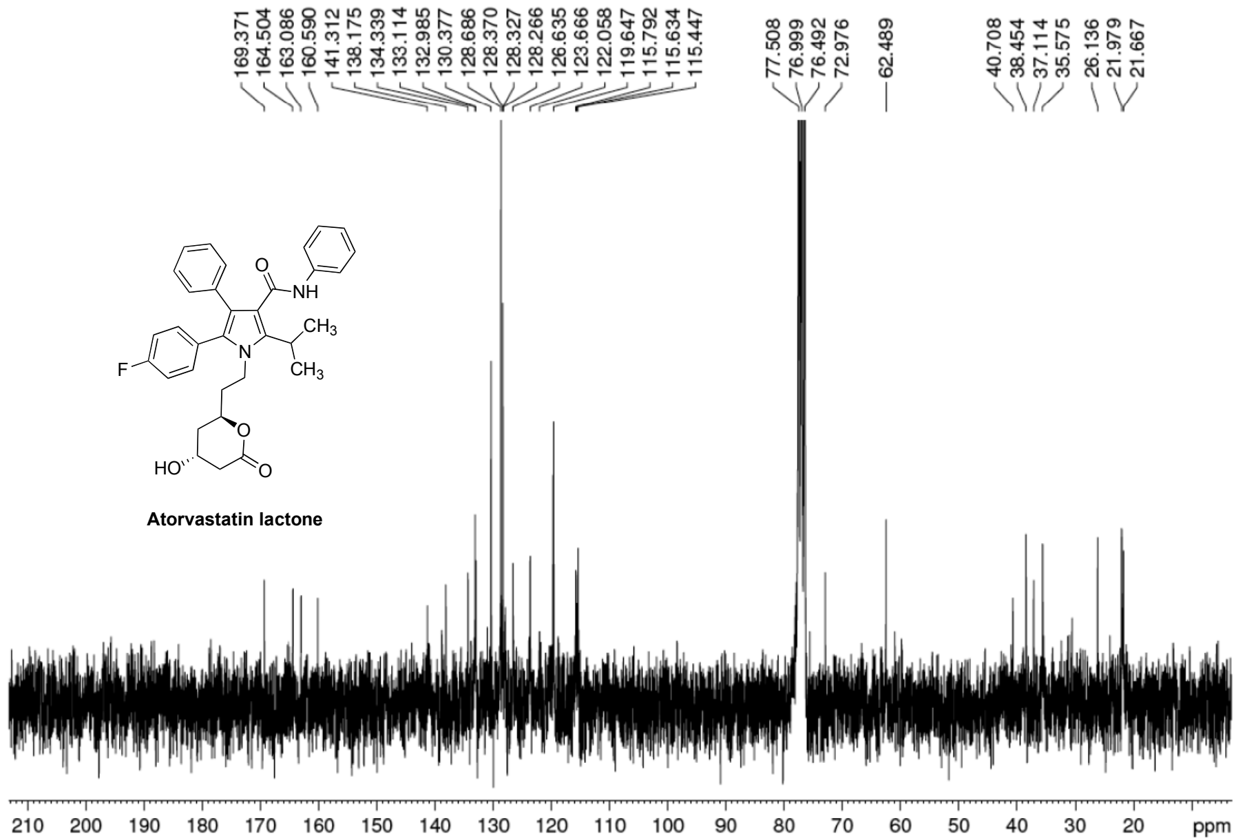
^{13}\text{C} NMR spectrum of atorvastatin lactone (9)
