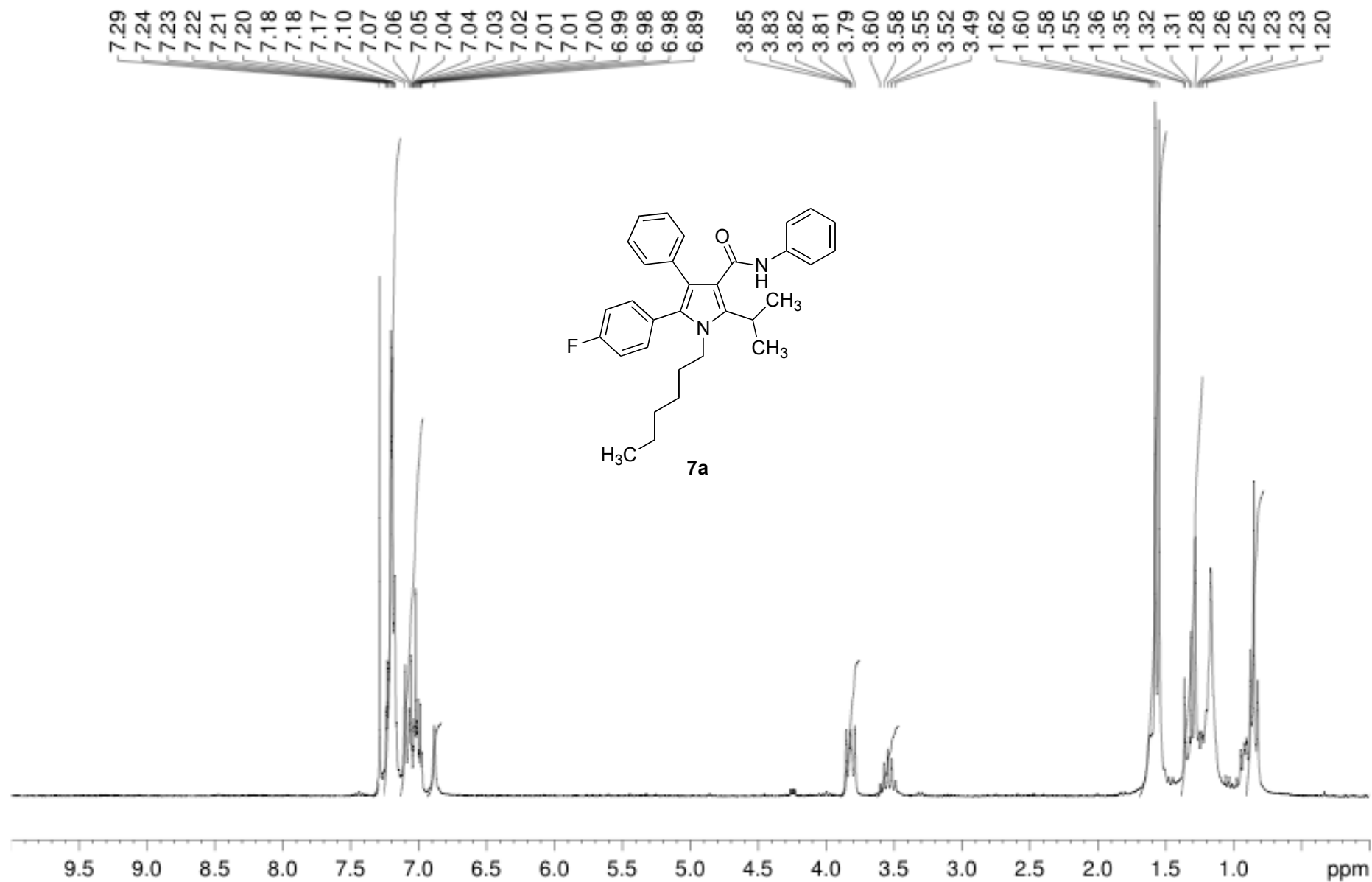
^1\text{H} NMR spectrum of compound 7a
