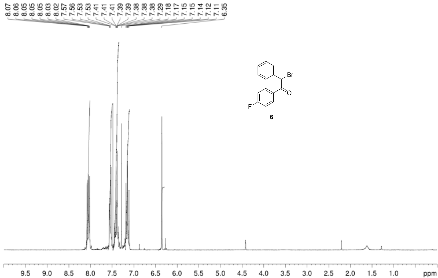
^1\text{H} NMR spectrum of compound 6
