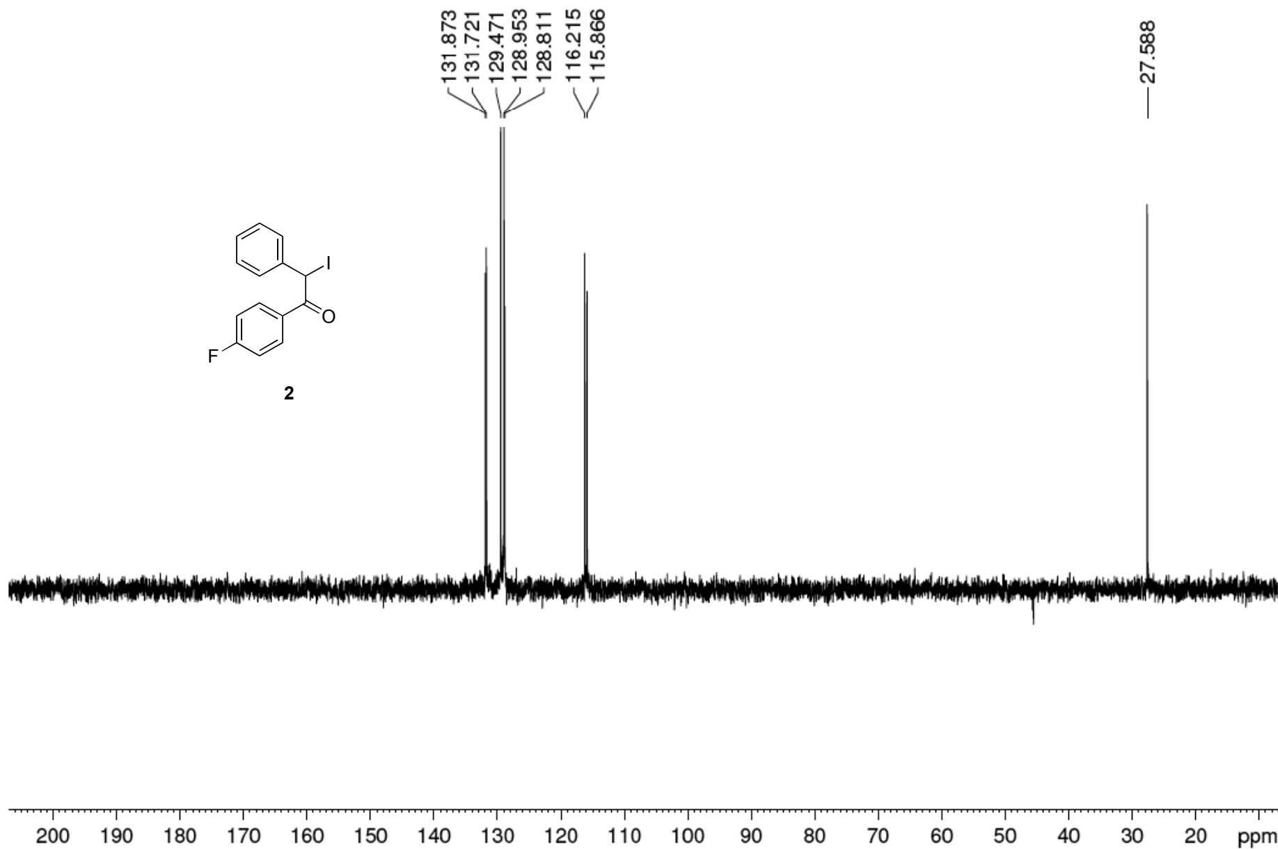
DEPT-135 spectrum of compound 2
