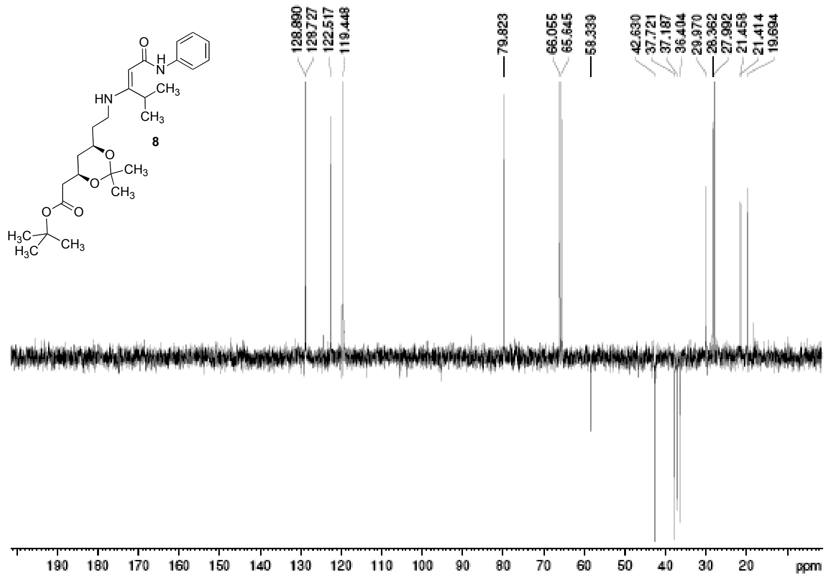
DEPT-135 spectrum of compound 8
