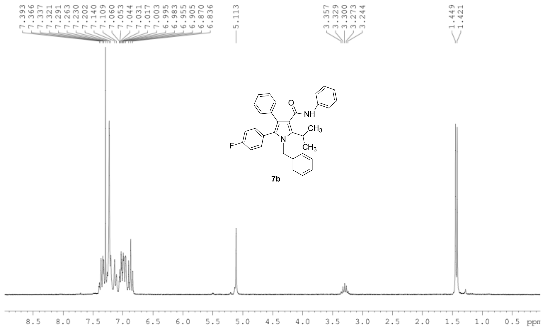
1 H NMR spectrum of compound 7b
