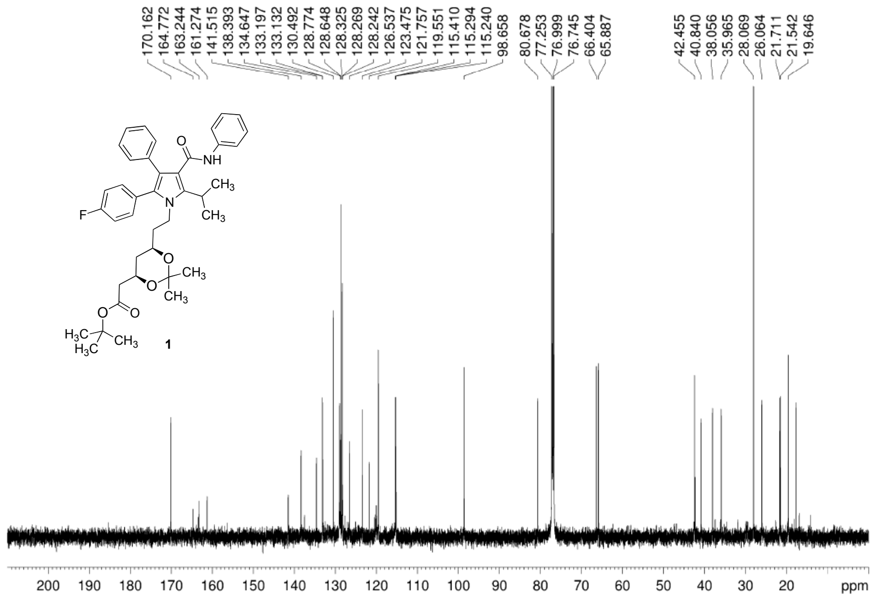
13 C NMR spectrum of compound 1
