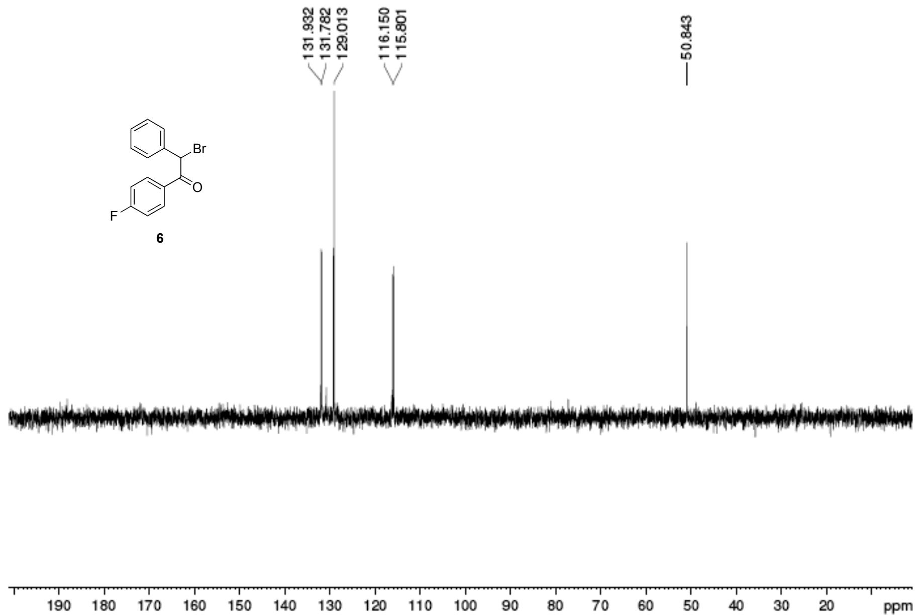
DEPT-135 spectrum of compound 6
