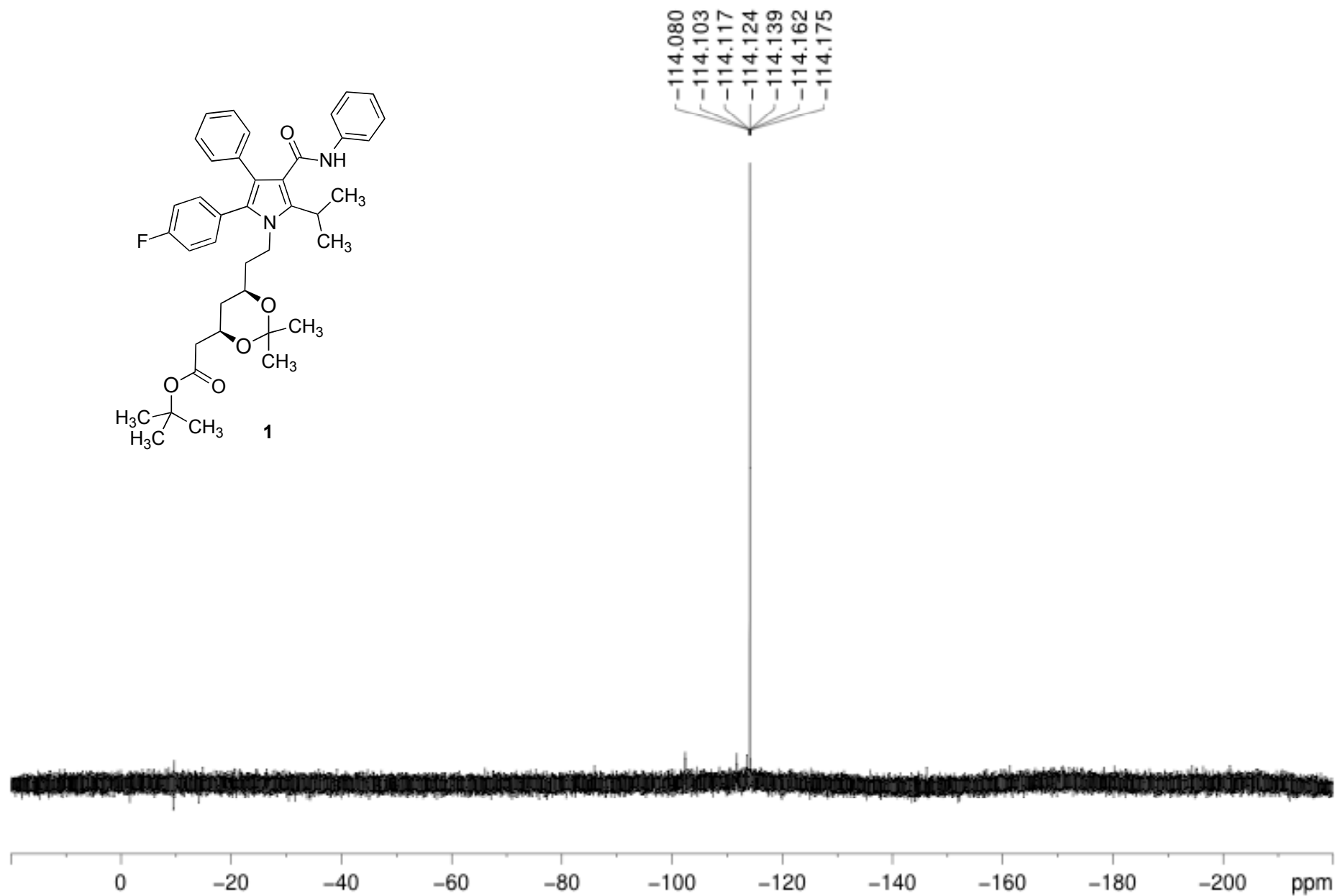
^{19}\text{F} NMR spectrum of compound 1 S24
