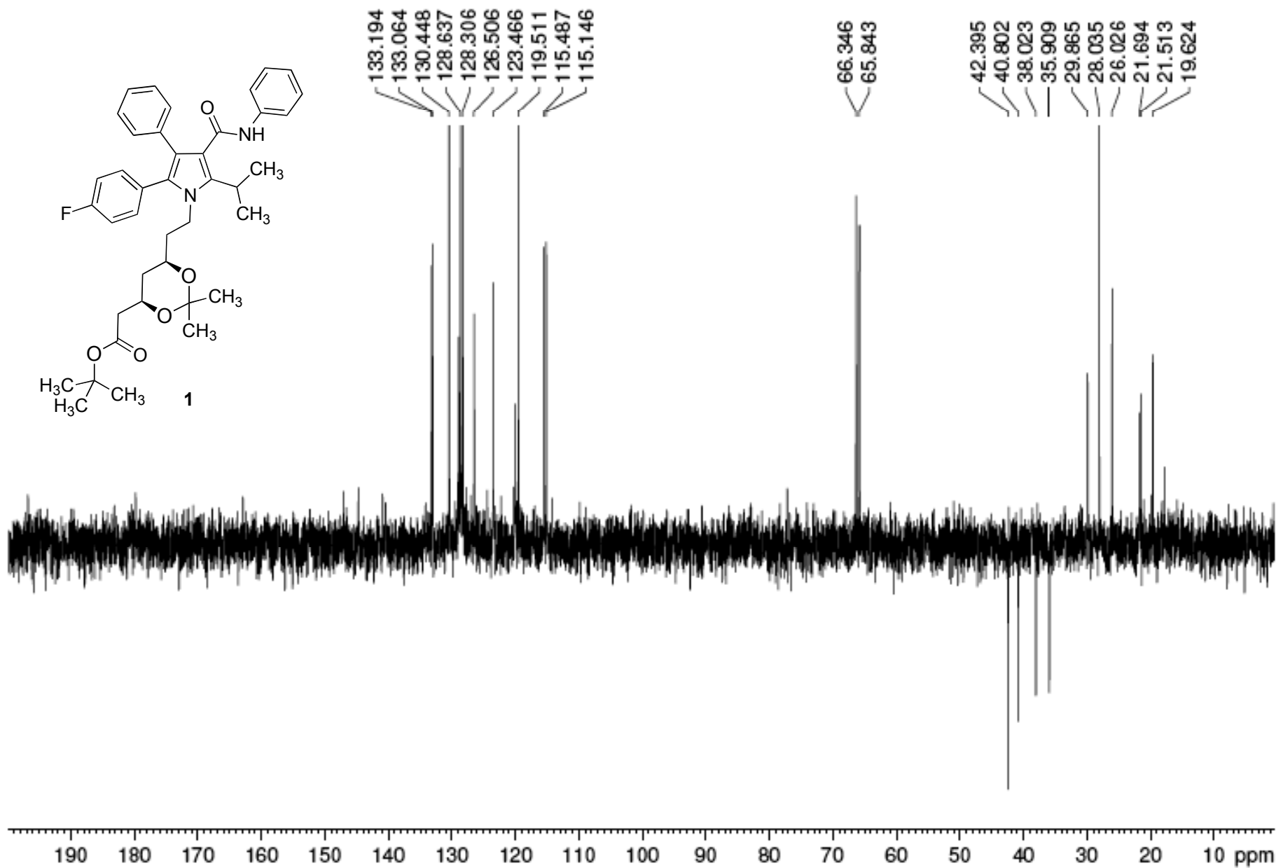
DEPT-135 spectrum of compound 1
