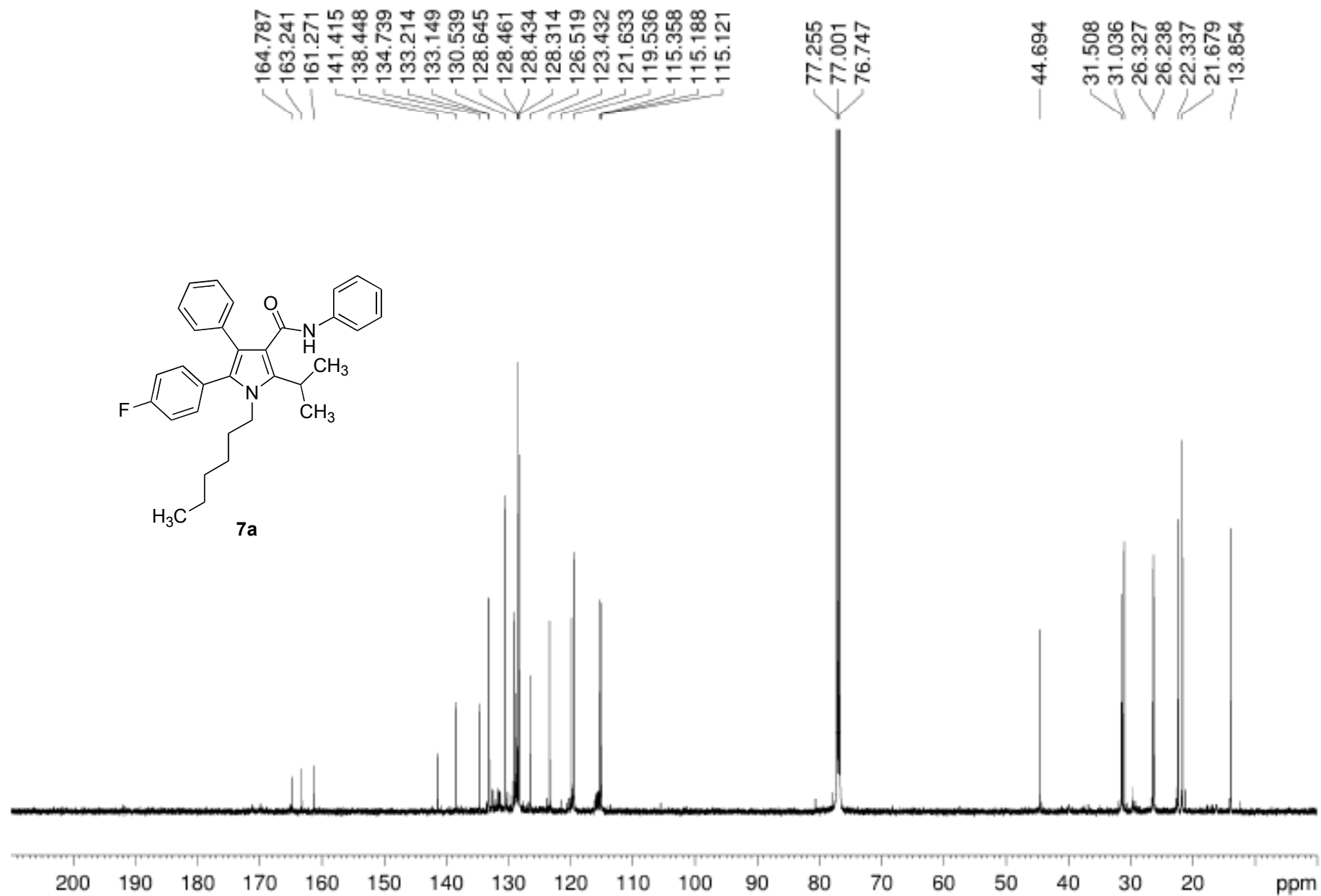
^{13}\text{C} NMR spectrum of compound 7a
