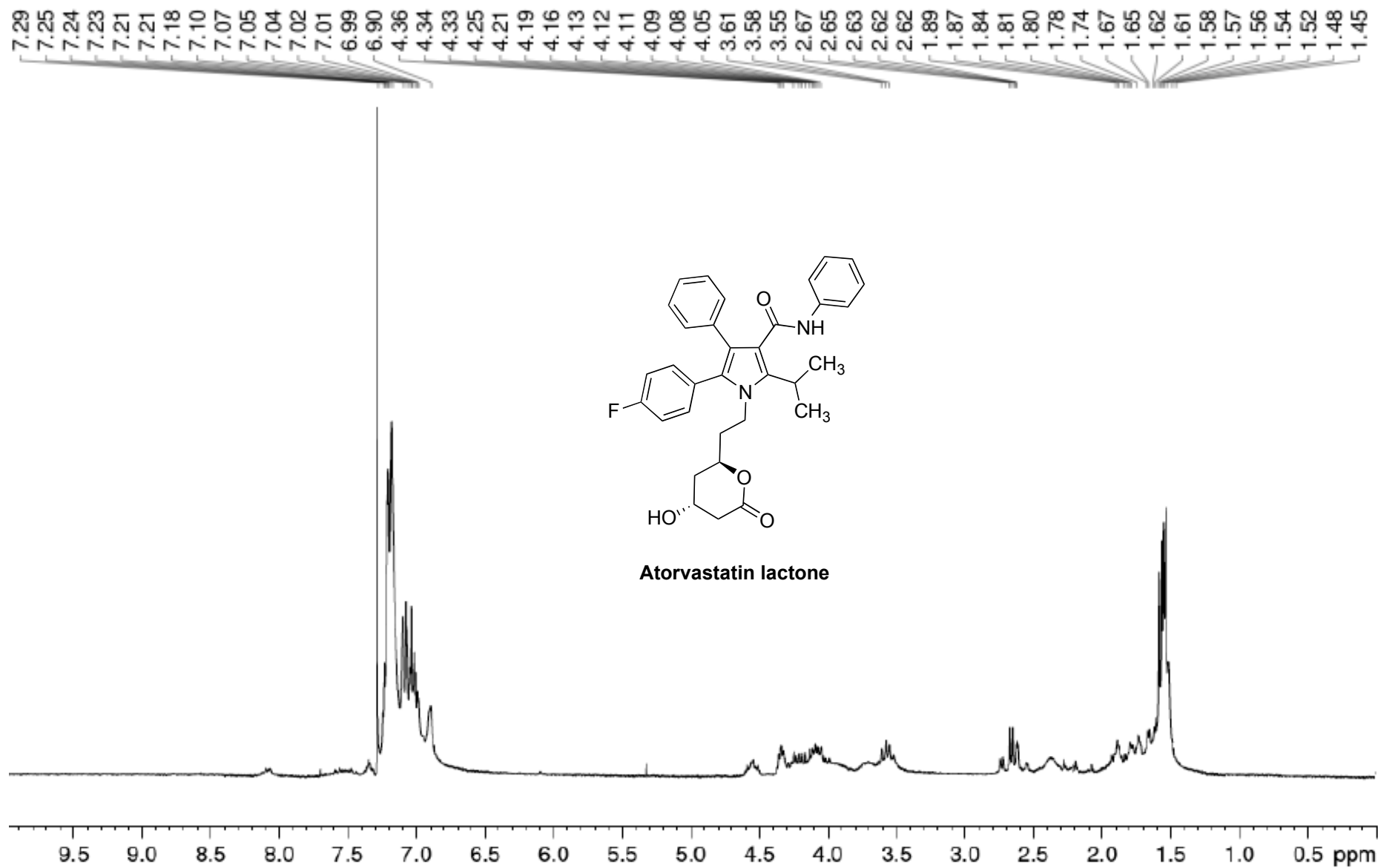
^1\text{H} NMR spectrum of atorvastatin lactone (9)
