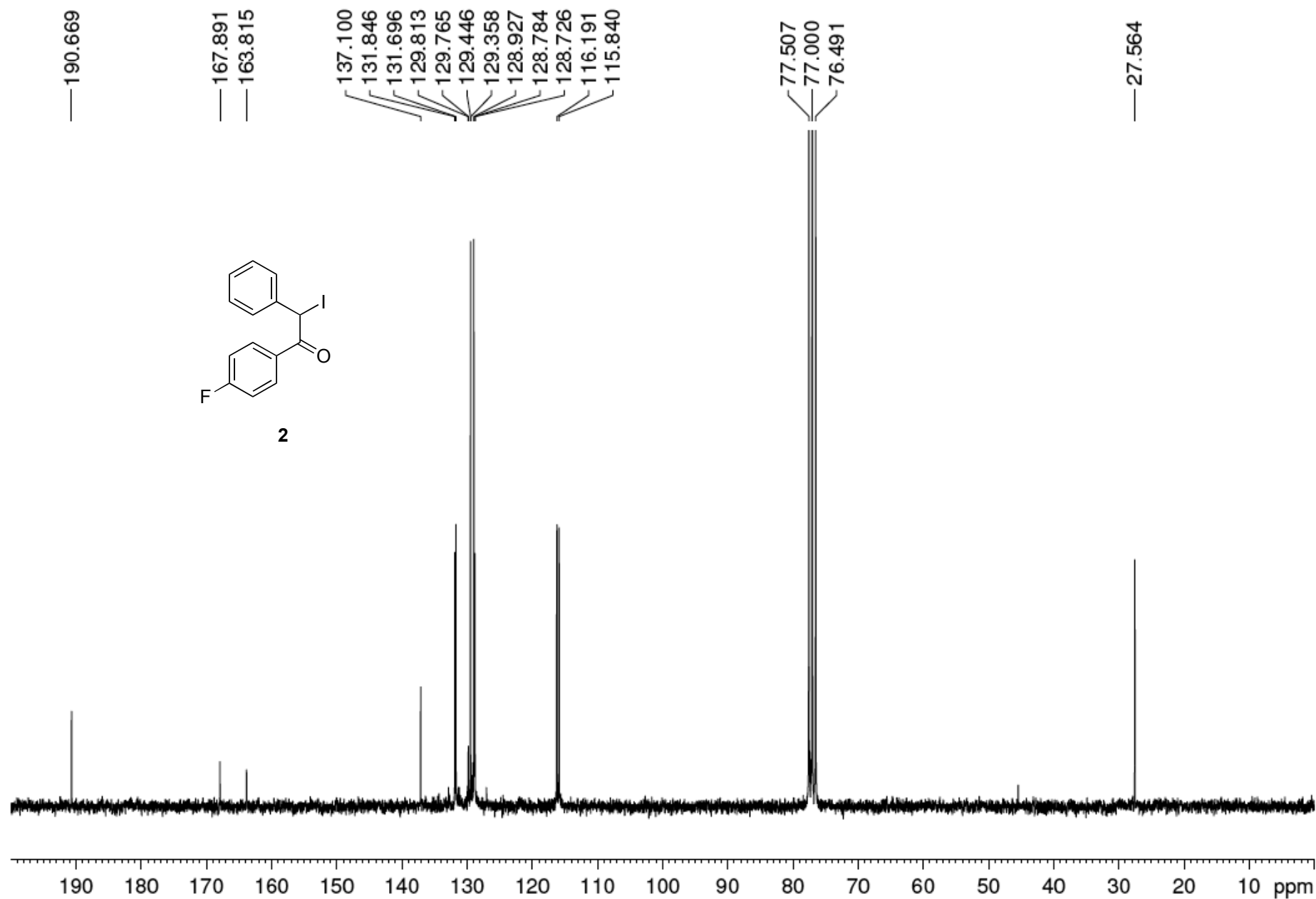
^{13}\text{C} NMR spectrum of compound 2
