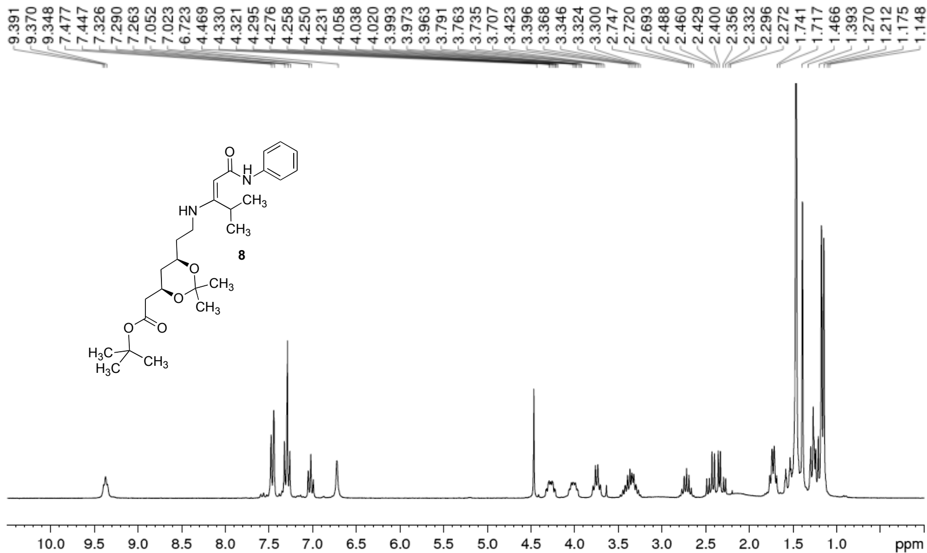
1 H NMR spectrum of compound 8
