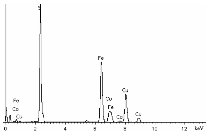
Supporting Figure 5c Energy-dispersive X-ray spectroscopy (EDS) of Sample12
