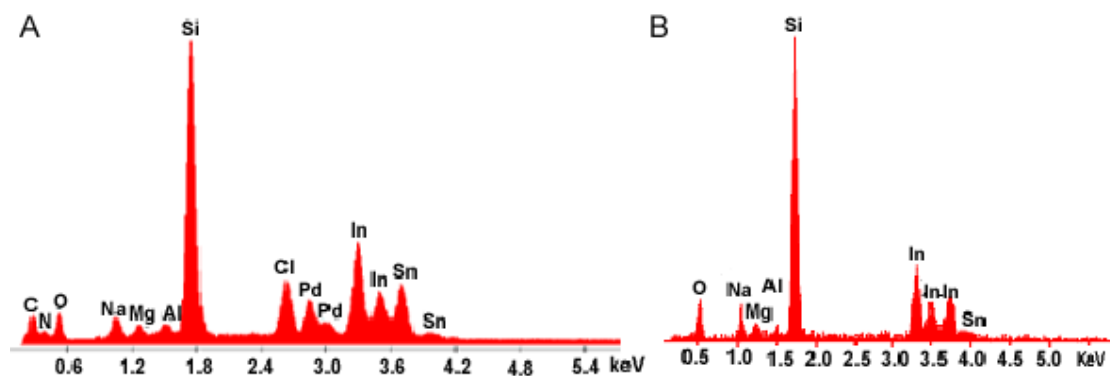
Fig. S1. Energy-dispersive spectrum of (A) microparticle-coated and (B) bare ITO substrate.
