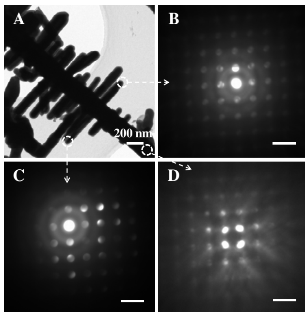
Fig.S1 A. TEM image of Sn nanodendrites; B-D. The micro-XRD patterns for the corresponding regions in TEM image.
