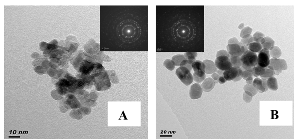
Figure 1S: TEM image of CeO 2 calcined at (A) 400 and B) 600 °C. The insets show the corresponding SAED diffraction patterns.
