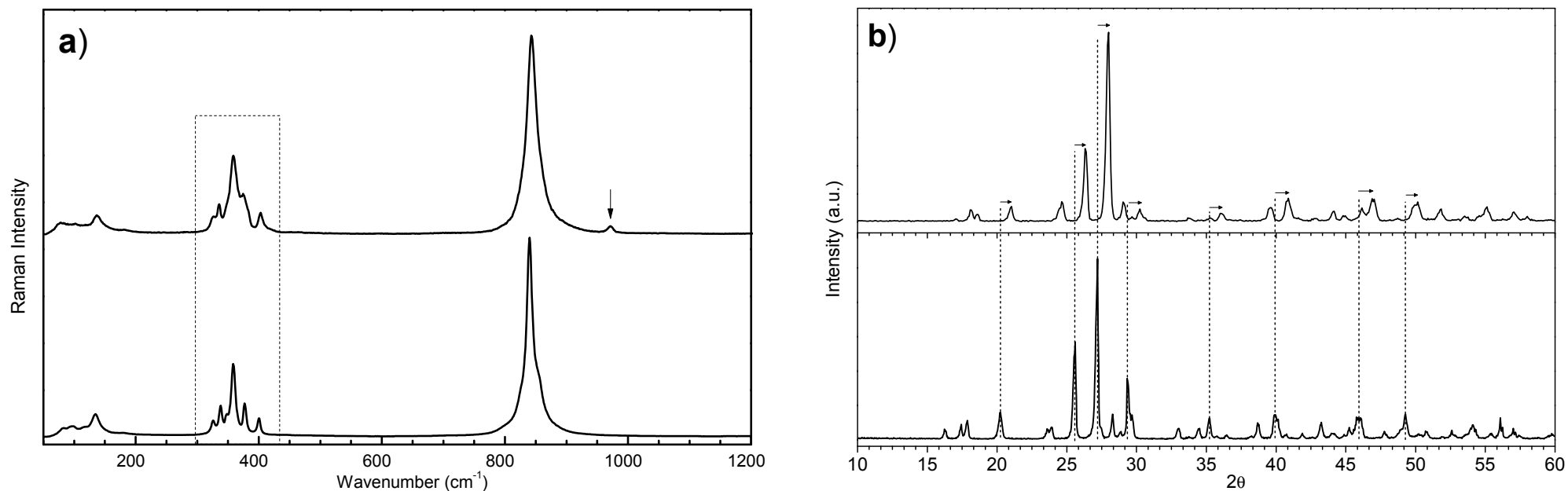
Fig. A.1 a) Raman spectra of PbCrO 4 below and Pb(Cr,S)O 4 on top, and b) Diffractograms of PbCrO 4 below and Pb(Cr,S)O 4 on top (JCPDS: 01-73-1332). The differences due to the introduction of sulfur ions in the crystalline structure of crocoite may be observed. See text for more details.
