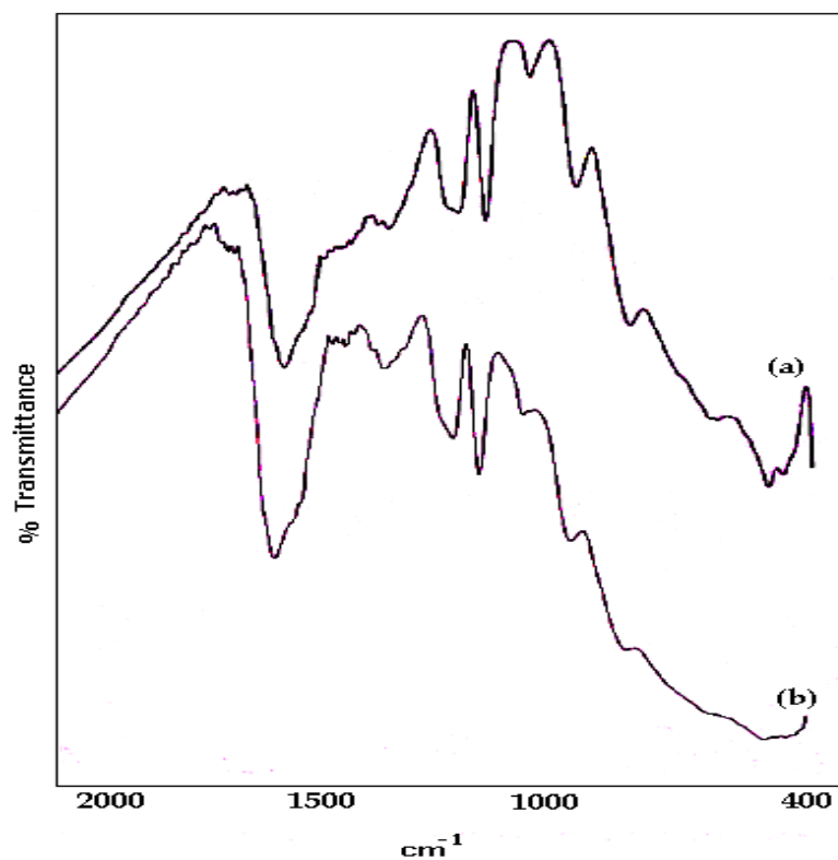
Fig.S1. FT-IR of (a) TPA/ZrO 2 and (b) PdTPA/ZrO 2
