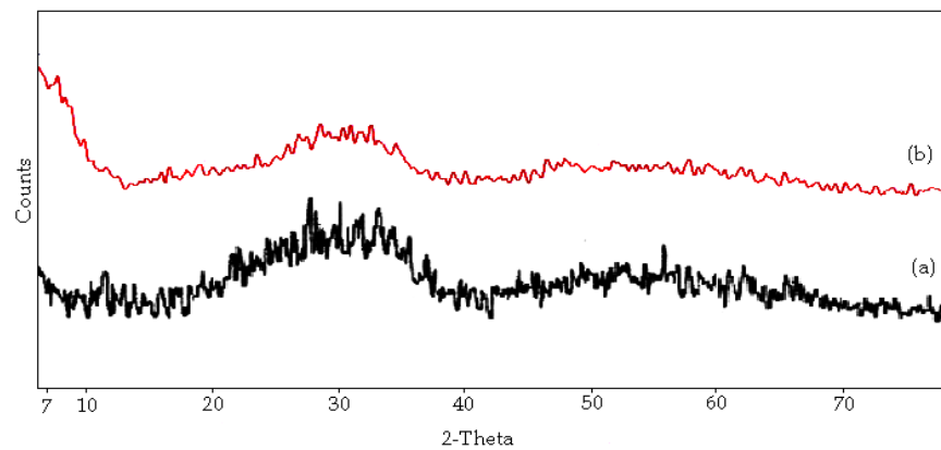
Fig.S2 XRD of (a) TPA/ZrO 2 and (b) Pd-TPA/ZrO 2
