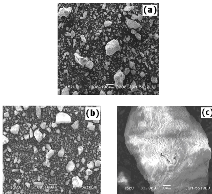
Fig. S3. SEM of (a) TPA/ZrO 2 (100x), (b) Pd-TPA/ZrO 2 (100x) and (c) Pd-TPA/ZrO 2 (1000x)
