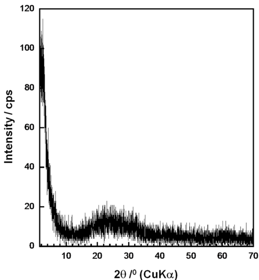
Figure S1. XRD pattern of as-synthesized titanium oxide-ODA hybrid particles.
