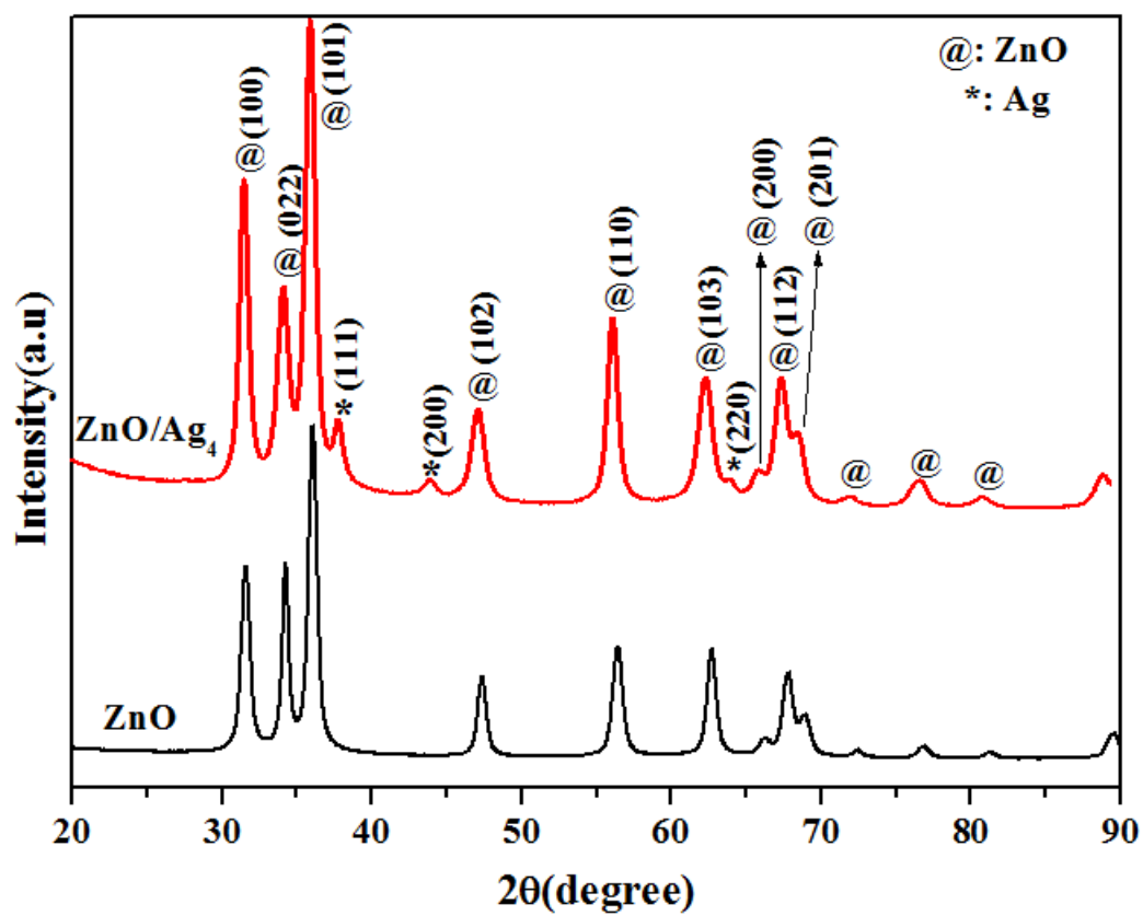
Fig. S1 Slow scan powder XRD pattern of ZnO and ZnO/Ag 4 .
