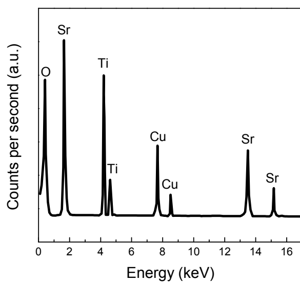
Fig. S2 EDS image of the mesoporous SrTiO 3 NWs synthesized at Ti/Sr = 1:1.05.
