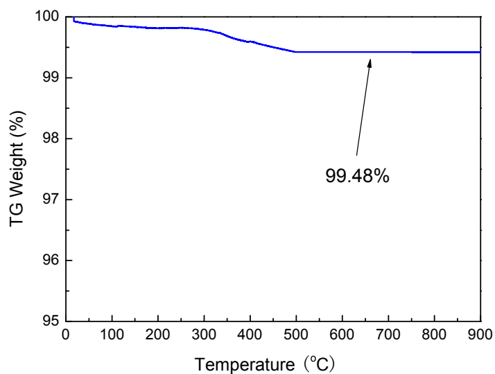
Fig. S1 The TG curve of the mesoporous SrTiO 3 NWs synthesized at Ti/Sr = 1:1.05.
