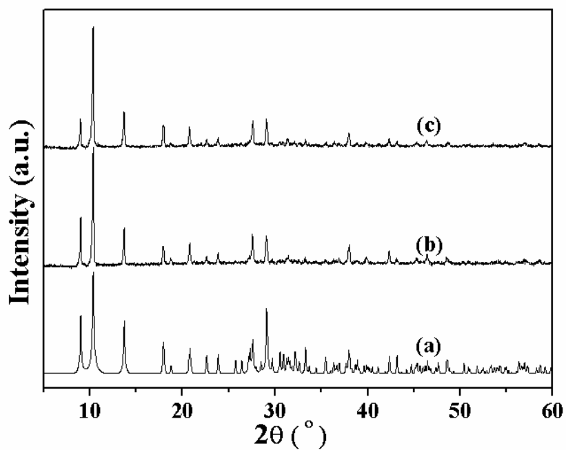
Fig. S4 XRD patterns of Cu-MOF: (a) calculated Cu-MOF, (b) fresh Cu-MOF and (c) used Cu-MOF after cyclohexene oxidation.
