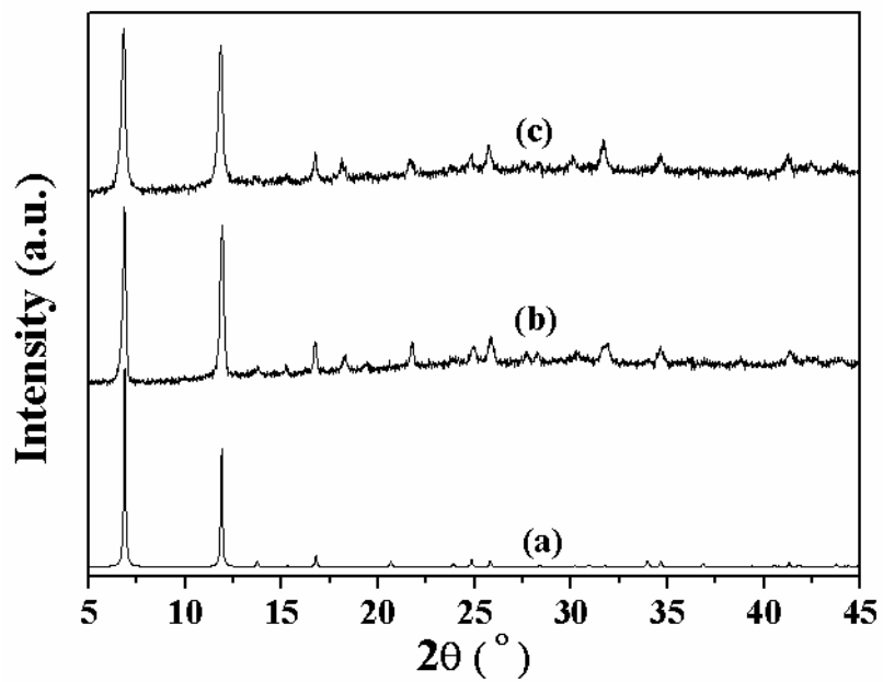
Fig. S3 XRD patterns of Co-MOF: (a) calculated Co-MOF, (b) fresh Co-MOF and (c) used Co-MOF after cyclohexene oxidation.
