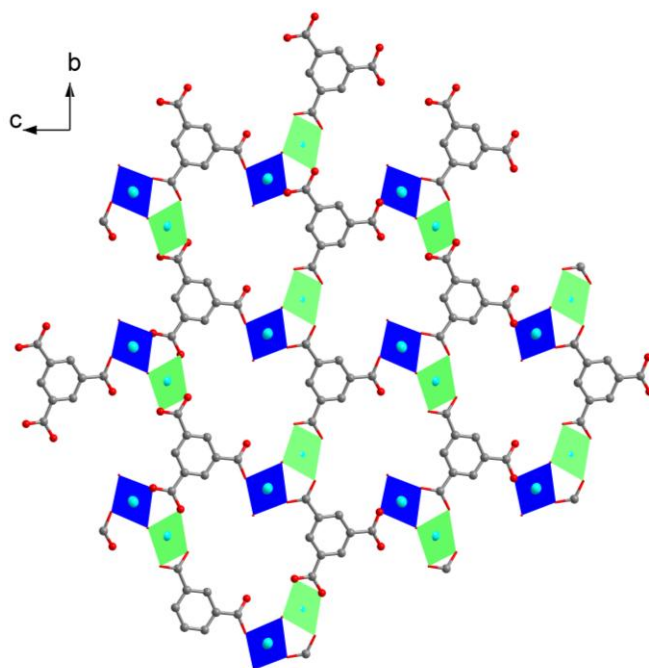
Fig. S1 A schematic drawing of the structure of Cu-MOF.
