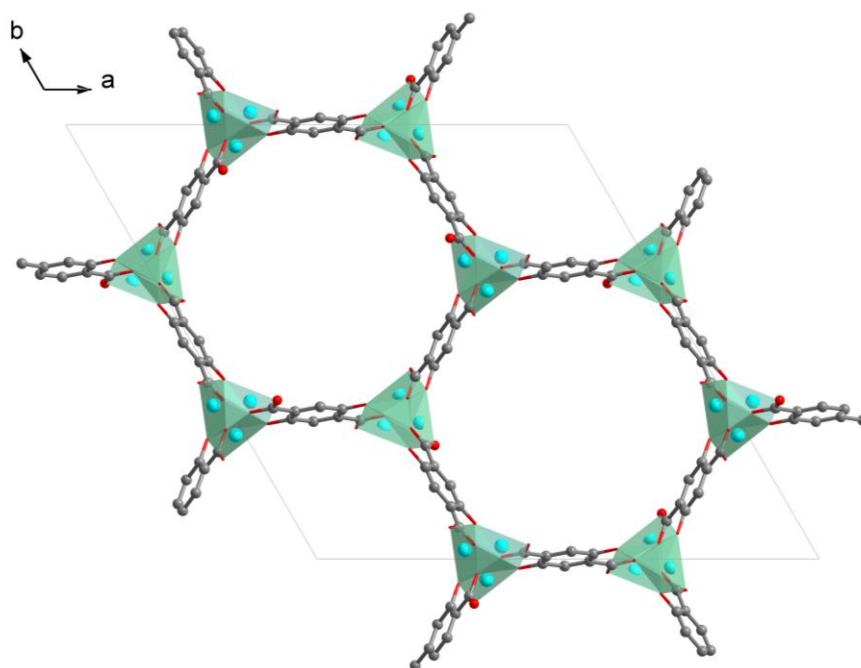
Fig. S2 A schematic drawing of the structure of M-MOF (M=Co or Ni).
