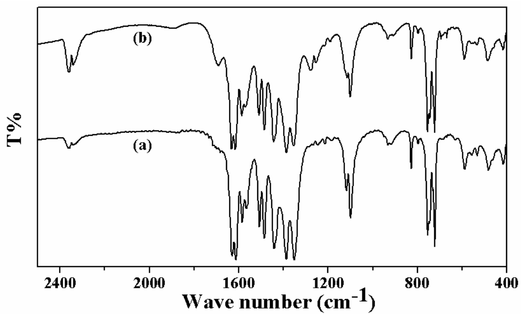
Fig. S6 IR spectra of Cu-MOF (a) before and (b) after oxidation of cyclohexene.
