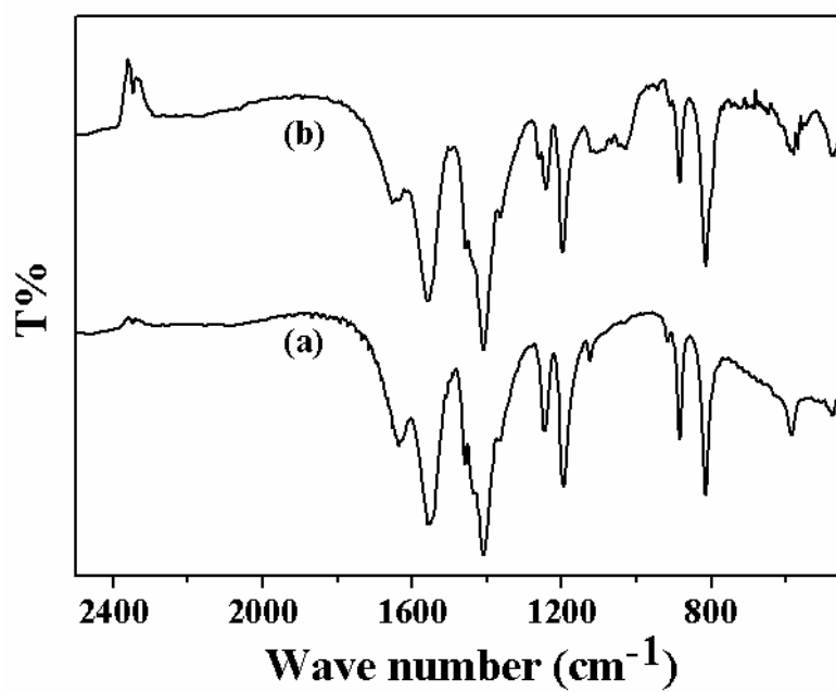
Fig. S5 IR spectra of Co-MOF (a) before and (b) after oxidation of cyclohexene.
