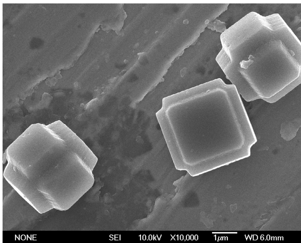
Fig. S1. SEM image of elongated PB microcrystals.
