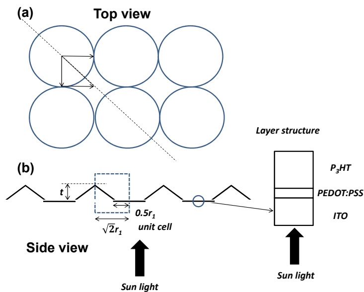
Figure S1 Schematic configuration of 2D-NBRs for simulation with (a) top and (b) side views.
