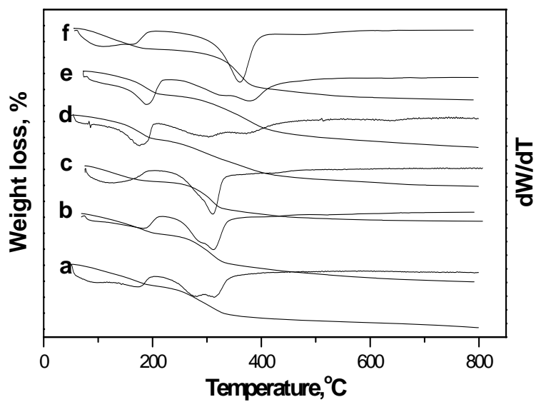
Figure S2. TG-DTG curves of: (a) NiAl 2 , (b) NiAl 3 , (c) NiAl 4 , (d) MgAl 2 , (e) MgAl 3 , (f) MgAl 4
