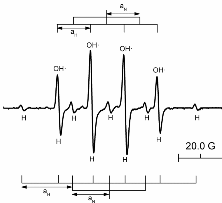
Figure S2. EPR spectrum of spin adducts DMSO-OH from our X-ray irradiated
