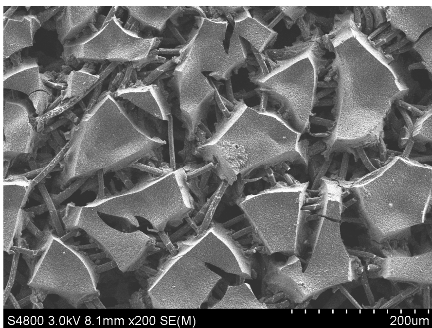
Fig. S1 SEM image of the CAGs/SMF-Ni electrode sample.
