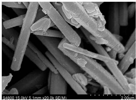
Fig. S1 FE-SEM image of ZnO nanorods.
