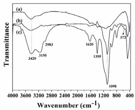
Fig. S2 FT-IR spectra of ZnO nanorods (a), ZnO/SiO 2 (b), ZnO-Br (c).
