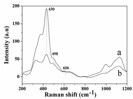
Fig. S3 Raman spectra of ZnO-MIPs (a) and ZnO-NIPs (b).
