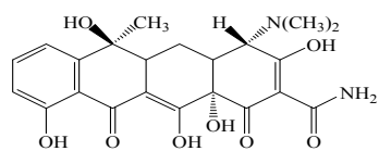
Tetracycline (TC)
