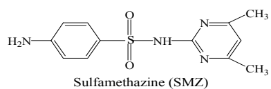
Sulfamethazine (SMZ)
