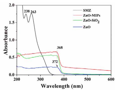
Fig. S4 UV-vis adsorption spectra of SMZ, ZnO-MIPs, ZnO-SiO 2 and ZnO.
