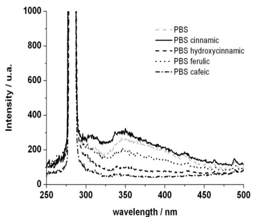
Figure S.I.2. Fluorescence spectra of PBS organic blends (a) and PBS nanocomposites (b) after 70 hours of irradiation.
