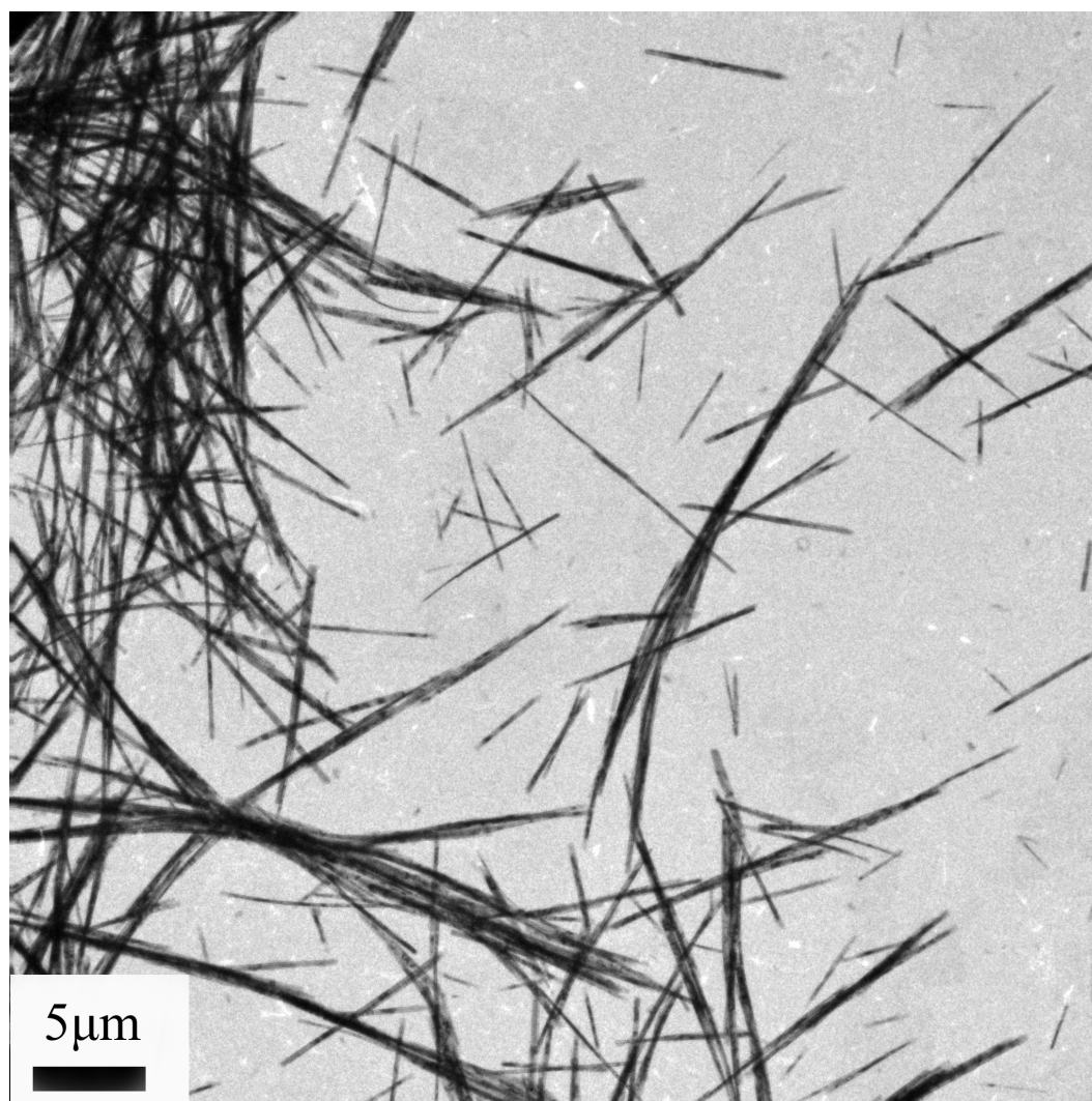
Figure S1. TEM image of the VO 2 (A) nanowires which obtained by hydrothermal treatment at 260°C for 16 h in the presence of 0.1mol/L VOSO 4 .
