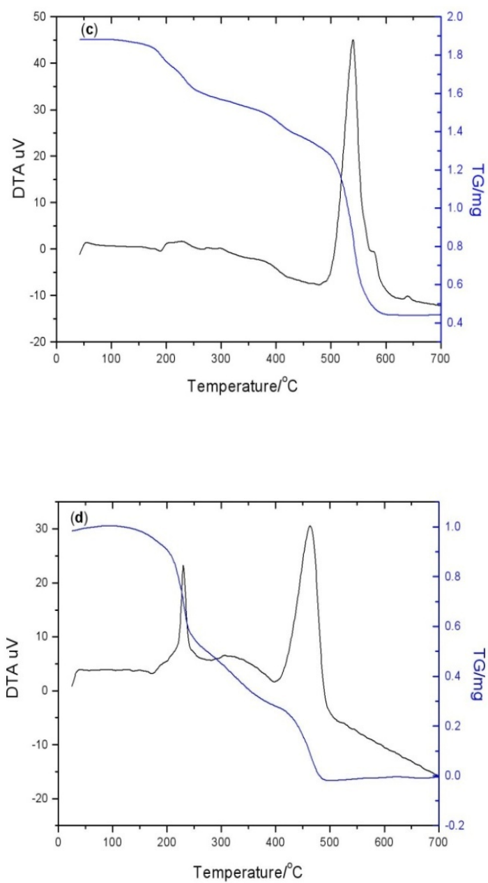
Fig. S1 Thermogravimetric analysis (TG/DTA) of salen ligand, (1), (2) and (3) complexes.
