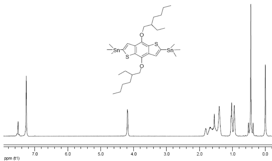
Figure S1 1 H NMR spectra of 2, 6-bis (trimethyltin)-4, 8-di(2-ethylhexyloxy) benzo[1,2-b:3,4-b']dithiophene , M1 , M2 and M3 .
