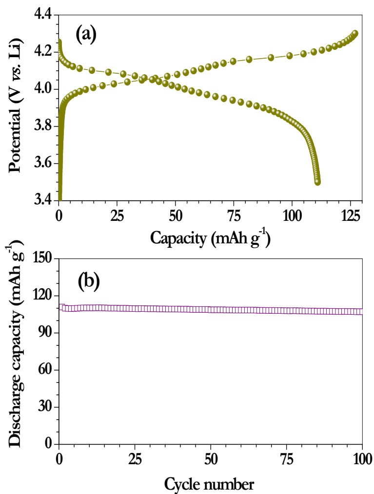
Figure Galvanostatic cycling performance (a) First charge-discharge curves of \text{Li}/\text{LiMn}_2\text{O}_4 cell between 3.5-4.3 V at current density of 150 \text{ mA g}^{-1} and (b) Plot of discharge capacity vs. cycle number (100 cycles)
