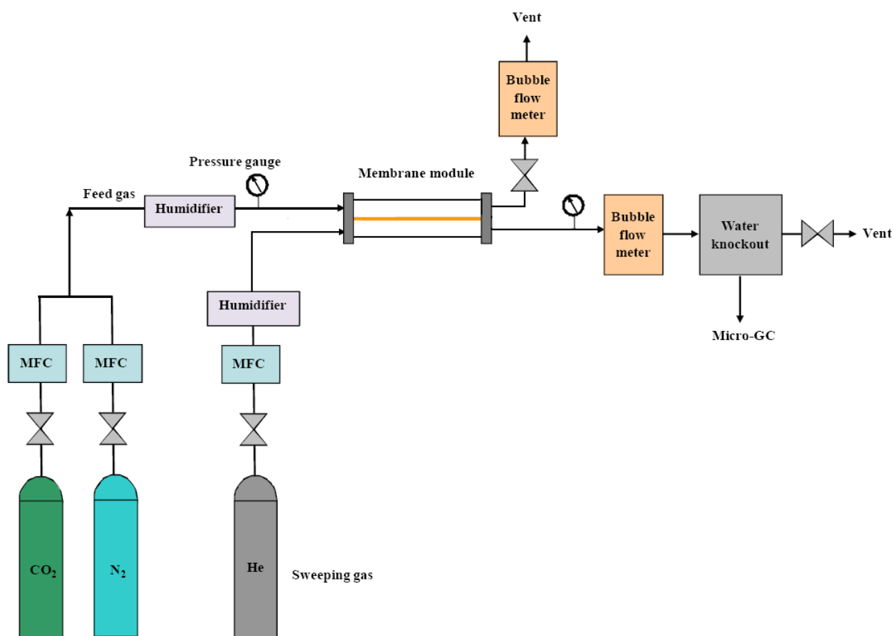
Figure S1. Experimental set-up for gas permeation test.
