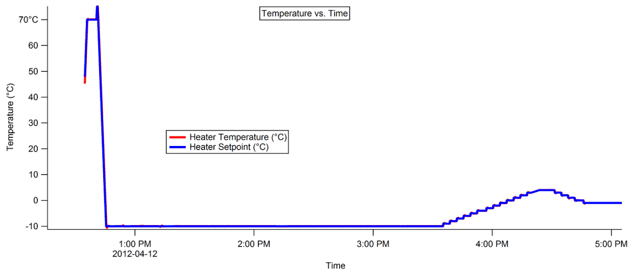
Graph 2. Temperature versus time dependence of the peltier cooler/heater stage used for taking Movie2 and Movie3. These movies demonstrate the melting and crystallization of 6CB/2% Gold system.
