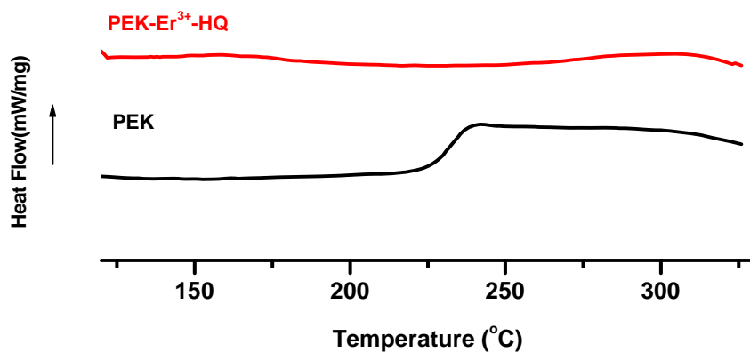
Fig. 1S DSC curves of PEK-1 and PEK-3-Er 3+ -HQ
