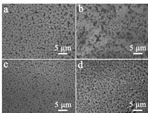
Fig. S2† FESEM images of product obtained with different etching time: (a) 0 h, (b) 0.5 h, (c) 1.5 h, (d) 5.5 h.
