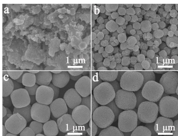
Fig. S1† FESEM images of product obtained with different hydrothermal time: (a) 1 h, (b) 3 h, (c) 6 h, (d) 12 h.
