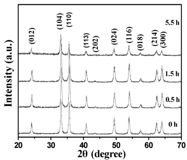
Fig. S3† XRD patterns of sample obtained with different etching time.
